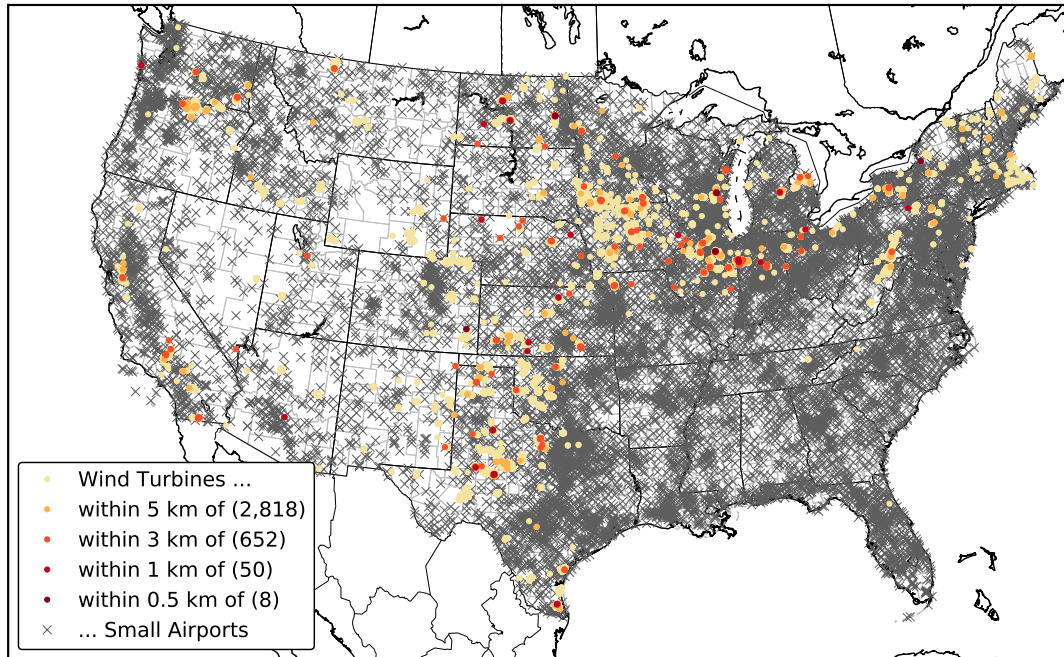
Figure 1. Map of wind turbines (dots) and small airports (x) in the continental United States. Turbines dots are colored increasingly red as their proximity to a small airport increases. The number of turbines in each distance range is shown in parentheses.
