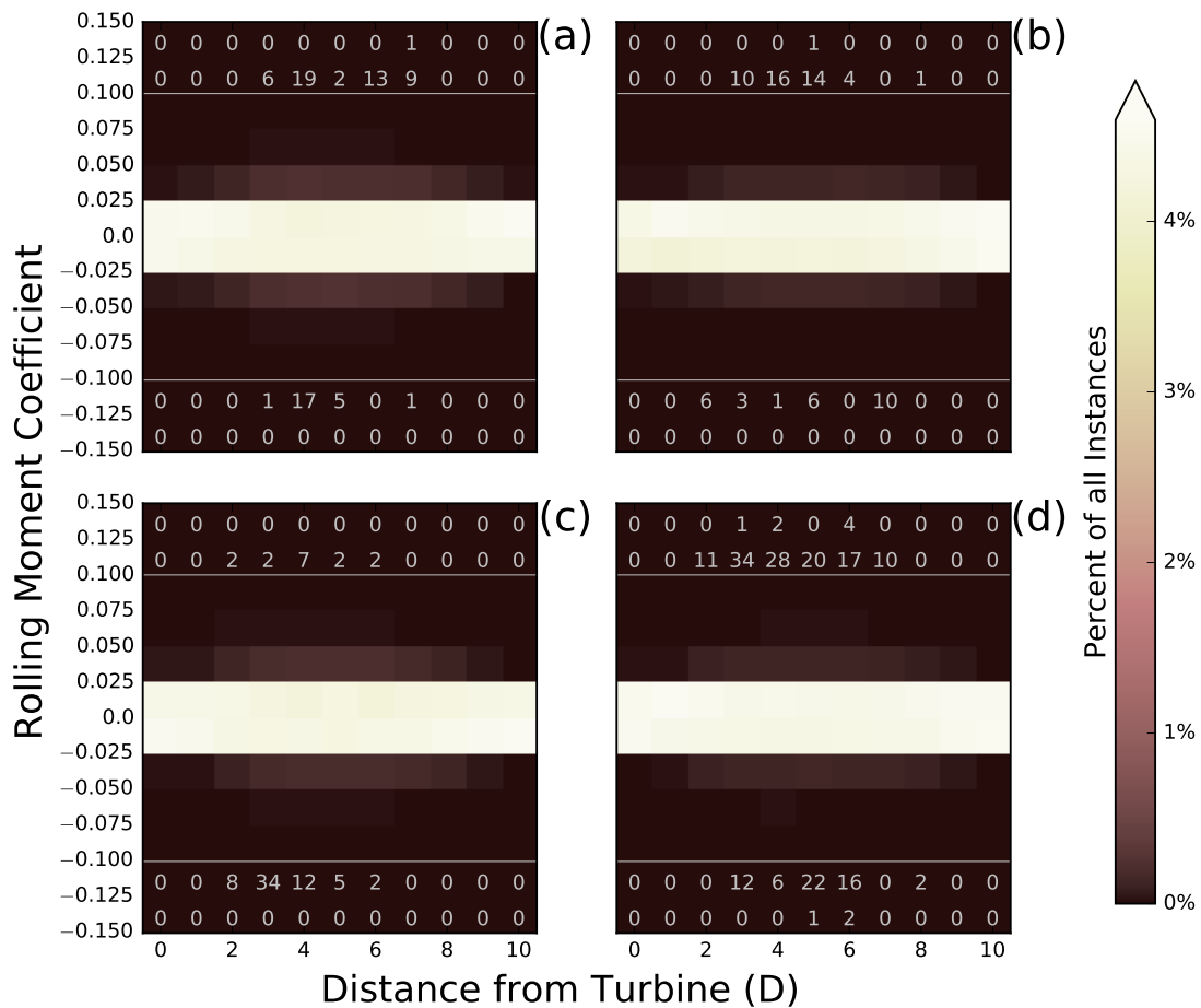
Figure 5. Two-dimensional histograms of all calculations of rolling moment coefficient experienced by all aircraft in the neutral (a, b) and stable (c, d) cases for down-wake (a, c) and cross-wake (b, d) transects as a function of the downwind distance from the turbine (in rotor diameters D ). “Non-low” hazards ( |C_{roll}| > 0.1 ) are explicitly totalled in their respective bins.
