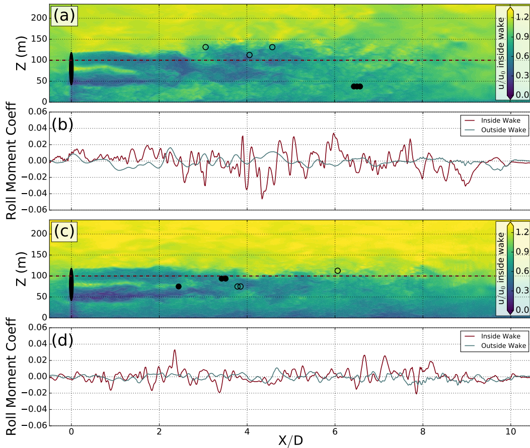
Figure 4. Comparison of rolling moment coefficient (b, d) between the flight path inside (red) and outside (blue) of the turbine wake in the neutral (a, b) and stable (c, d) cases. The vertical cross section of the downwind component of the wind velocity u , scaled by inflow wind speed u_0 , 7.4 and 9.4 \text{ m s}^{-1} in neutral and stable conditions, respectively, at the turbine location ( y = 0 ; a, c) is contoured for reference, over which the height of the flight paths ( z = 100 \text{ m} ) is traced in a red dashed line. The dots represent the downwind and vertical location of the three highest rolling moment coefficients experienced by the down-wake (black) and cross-wake (empty) array of aircraft.
