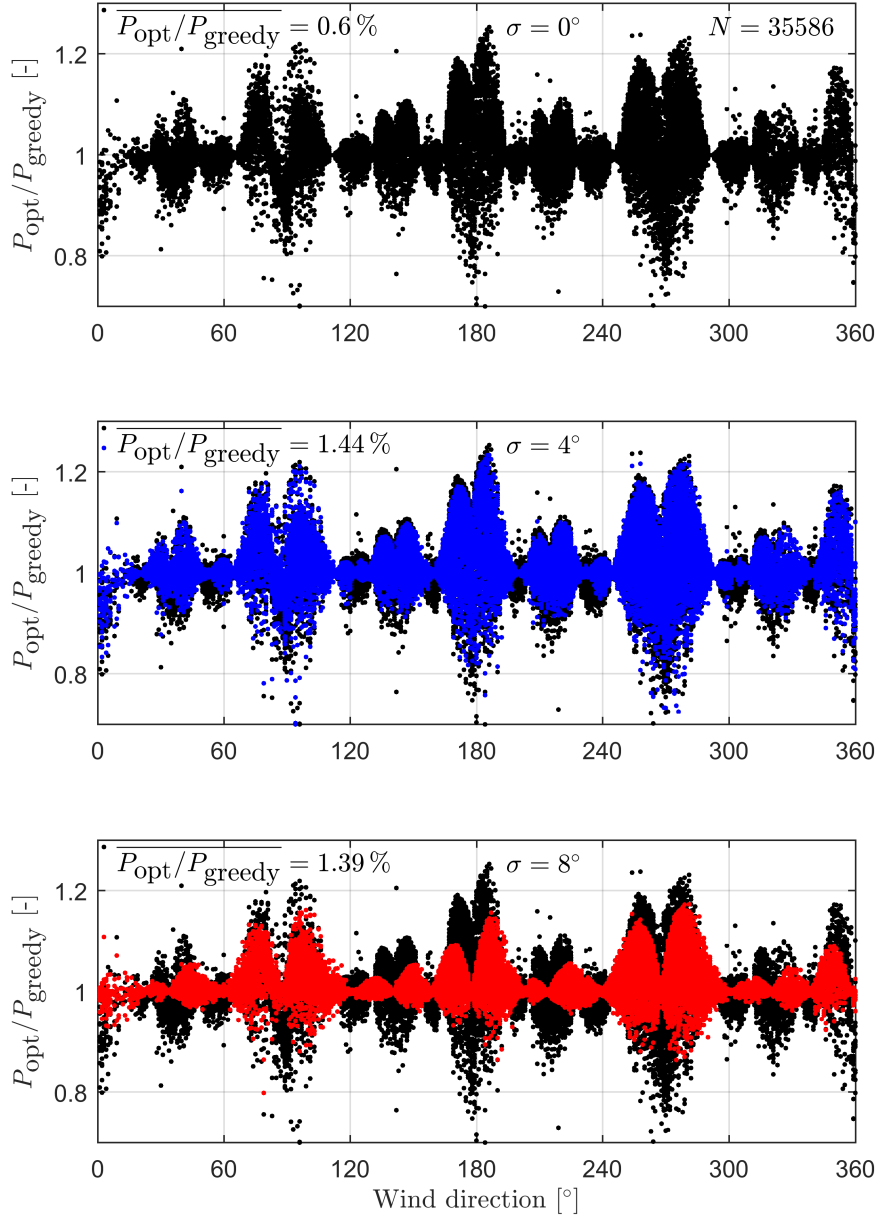
Figure 11. Test case A: Evaluation of the relative power gain over the estimated wind direction \varphi_{\text{est}} from the measured time series of 5 minutes averaged wind direction during a duration of approx. 5 months. a) conventional wake deflection (black), b) and c) robust wake deflection for \sigma = 4^\circ (blue) and \sigma = 8^\circ (red), respectively
