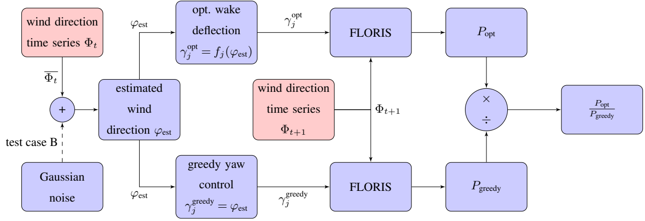
Figure 10. Evaluation process of the control schemes with wind direction measurements. Red boxes mark the steps in which the measured data is used as input.
