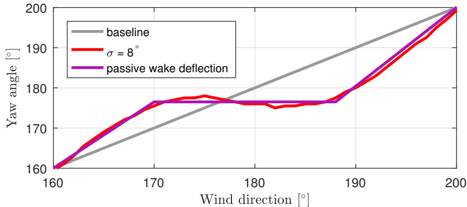
Figure 13. Exemplary illustration of the yaw angle set points of the reference turbine T32 according to the passive wake deflection.
