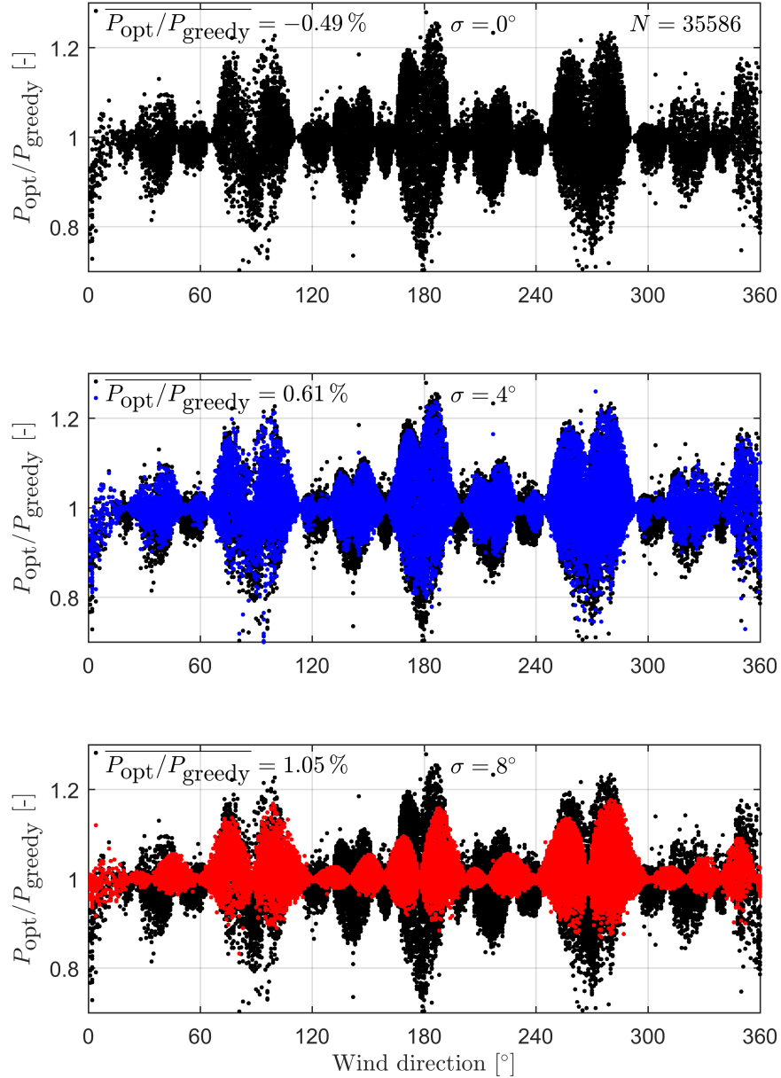
Figure 12. Test case B: Evaluation of the relative power gain over the estimated wind direction \varphi_{\text{est}} from the measured time series of 5 minutes averaged wind direction during a duration of approx. 5 months. a) conventional wake deflection (black), b) and c) robust wake deflection for \sigma = 4^\circ (blue) and \sigma = 8^\circ (red), respectively
