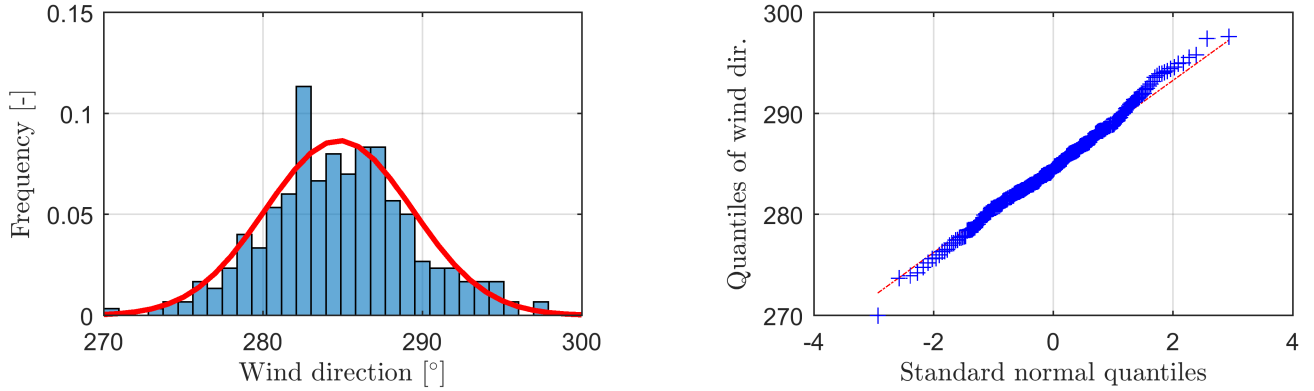
Figure 3. (left) Histogram of exemplary 5 min wind direction measurements, (right) quantile-quantile plot of the exemplary 5 min wind direction measurements
