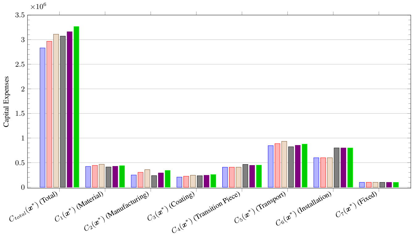
Figure 5. Expenses comparison of optimal solutions of three-legged jacket with three bays (light blue), three-legged jacket with four bays (light red), three-legged jacket with five bays (light tan), four-legged jacket with three bays (grey), four-legged jacket with four bays (purple), and four-legged jacket with five bays (green).
