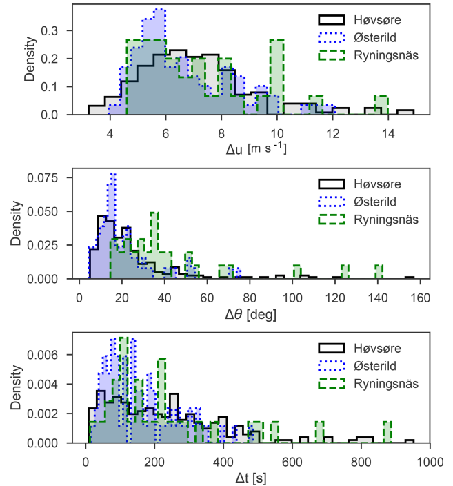
Figure 7. The distributions of detected amplitudes ( \Delta u ), direction changes ( \Delta\theta ), and rise times ( \Delta t ) of all the detected events at the three different sites: Høvsøre (grey), Østerild (blue), and Ryningsnäs (green).
