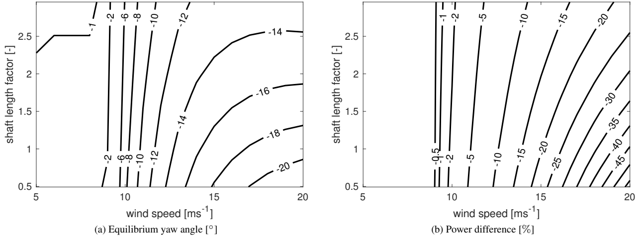
Figure 9. Equilibrium yaw angle (a) and the relative difference in power production (b) in dependency of shaft length and wind speed variation for a turbine configuration with 5^{\circ} tilt and 3.5^{\circ} cone. The relative, difference in power is compared at each calculation point relative to the power production of the original turbine, with a forced yaw alignment.
