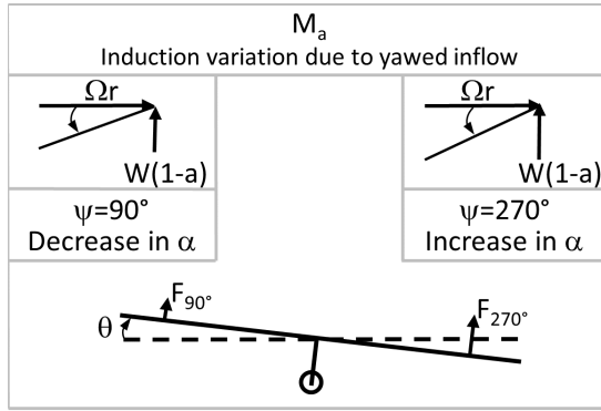
(a) Stiffness mechanism: induction variation.
