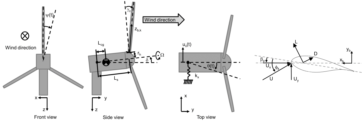
Figure 4. Schematics of turbine model and the according coordinate systems, front view, side view and top view (from left) and the sketch of the inflow and forces on the airfoil with the coordinate system.
