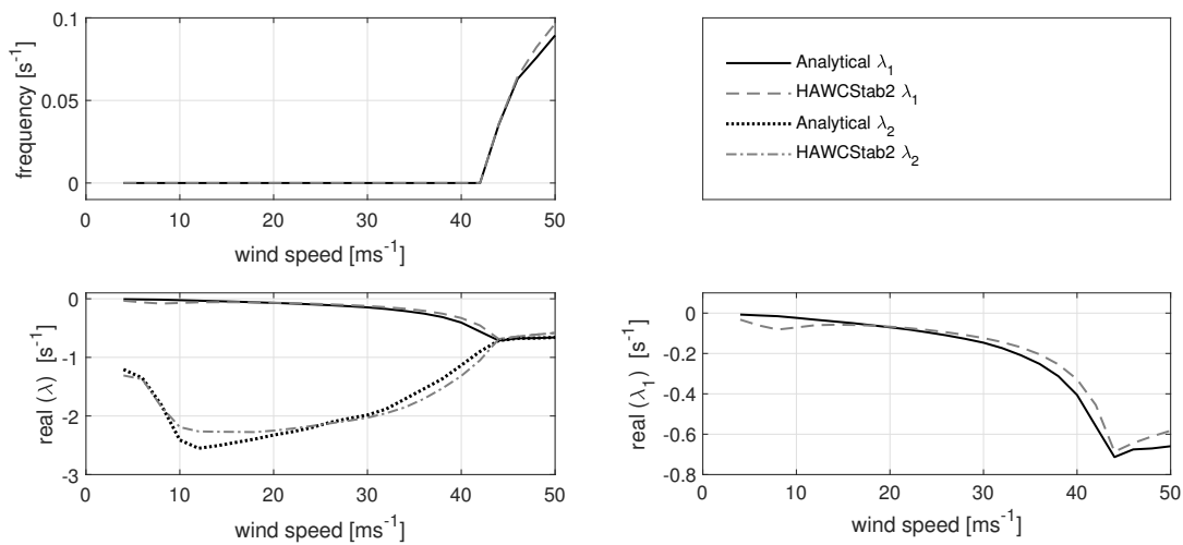
Figure 10. Comparison of the frequency (top left), the real part of the two eigenvalues (bottom left) and a zoom into the first eigenvalue (bottom right) of the yaw mode for the 2DOF model from the analytic solution, and the imitation in HAWCStab2.
