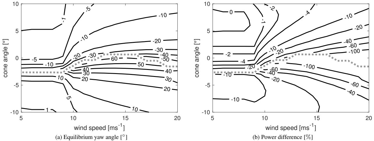
Figure 8. Equilibrium yaw angle (a) and the relative difference in power production (b) in dependency of cone angle and wind speed variation for a turbine configuration with 5^\circ tilt. The figure is stitched together from two sub-figures at the grey line.
