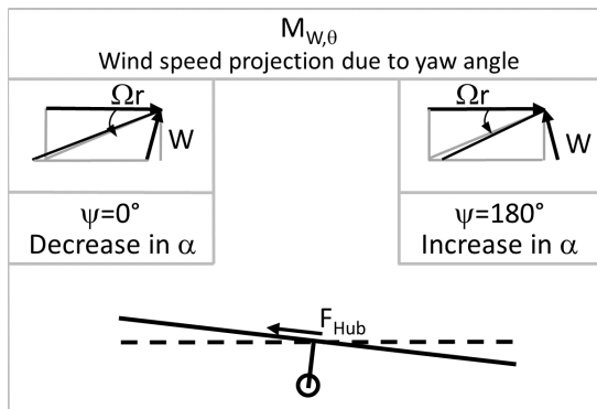
(c) Stiffness mechanism: yaw projection.
