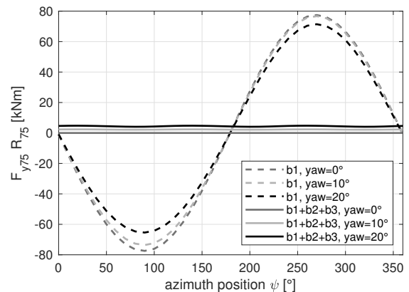
(f) Yaw moment estimate from F_y at R = 75\% and \gamma_c = 3.5^\circ .
