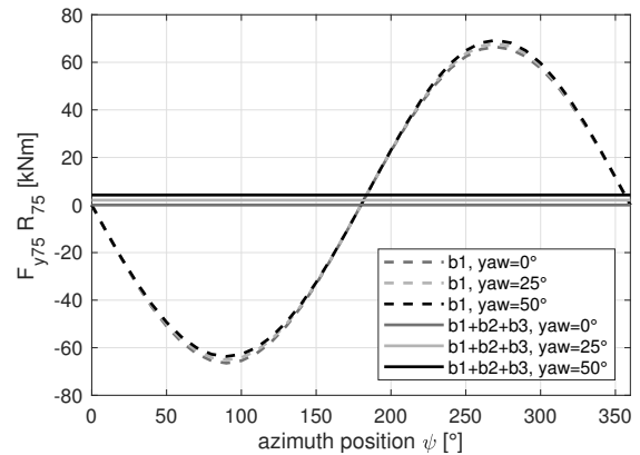
(b) Yaw moment estimate from F_y at R = 75\% .
