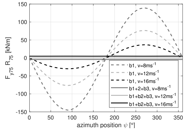
(b) Yaw moment estimate from F_y at R = 75\% and \delta=5^\circ .
