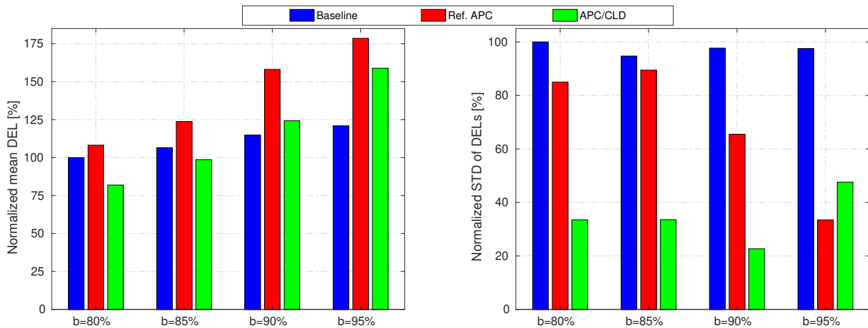
Figure 20. Normalized mean (left) and standard deviation (right) of the corresponding DELs of the tower base fore-aft bending moment for different levels of AGC power reference (23), parameterized as P_{\text{farm}}^{\text{base}} = 12.3 \text{ MW} , b = 80\% , 85\% , 90\% , 95\% , respectively, and c = 10\% . The baseline case with power demand level b = 80\% is considered as the reference.
