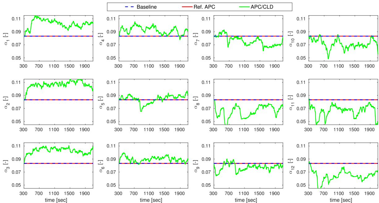
Figure 13. The trajectories of the power set-points with APC with coordinated load distribution (CLD). The baseline and Ref. APC rely on equal power set-points, i.e., \alpha_i = \frac{1}{12} .
