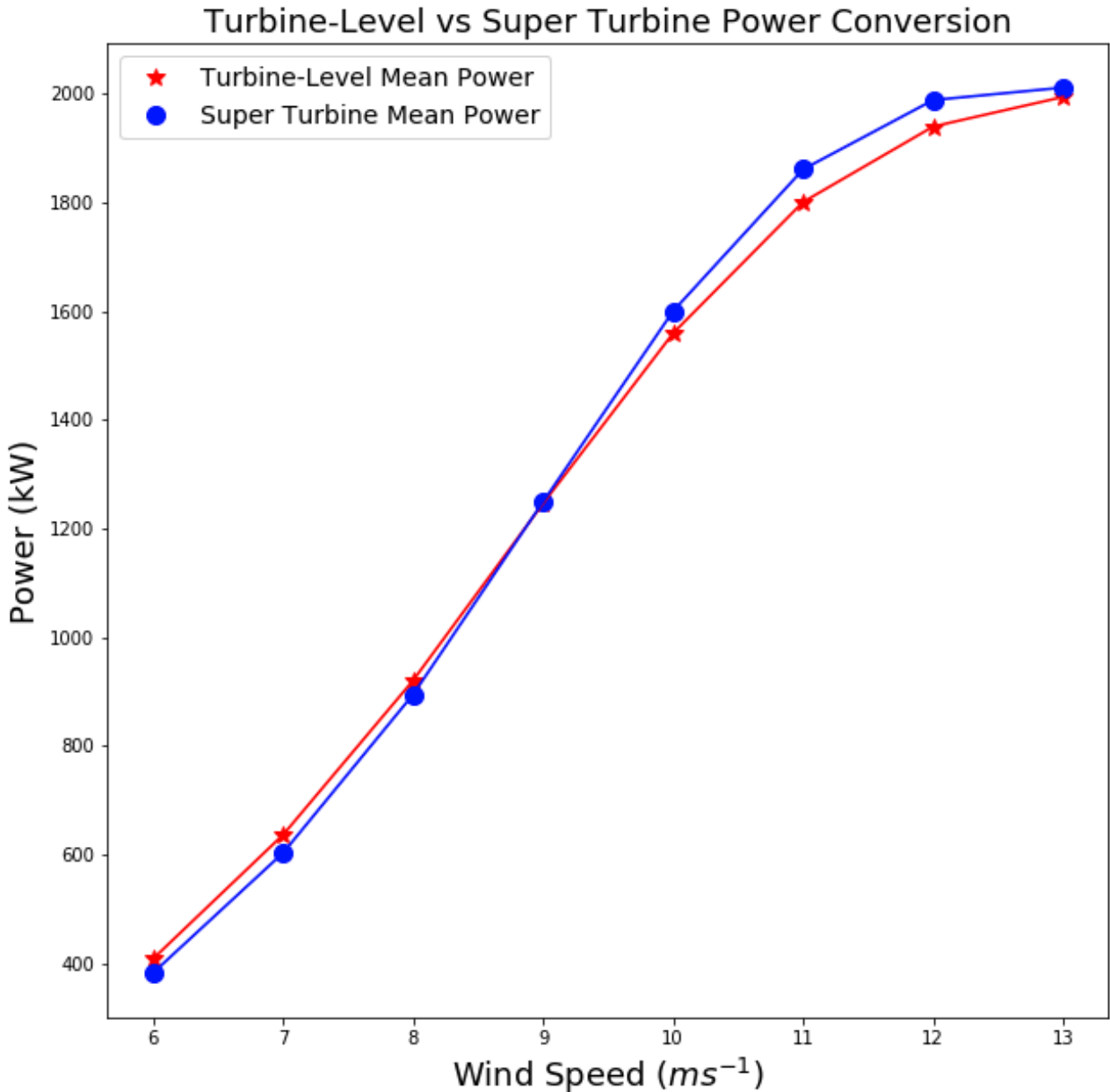
Figure 3: Comparison of the turbine-level power conversion to the super-turbine power conversion for the hypothetical wind farm with 1 m s^{-1} standard deviation across the turbines.
