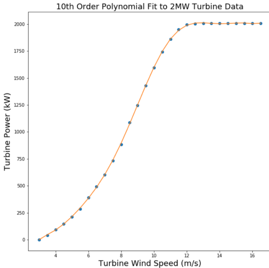
Figure 2: 10 th -order polynomial fit (orange line) to 2 MW Vestas turbine data from https://en.wind-turbine-models.com/turbines/16-vestas-v90#powercurve .
