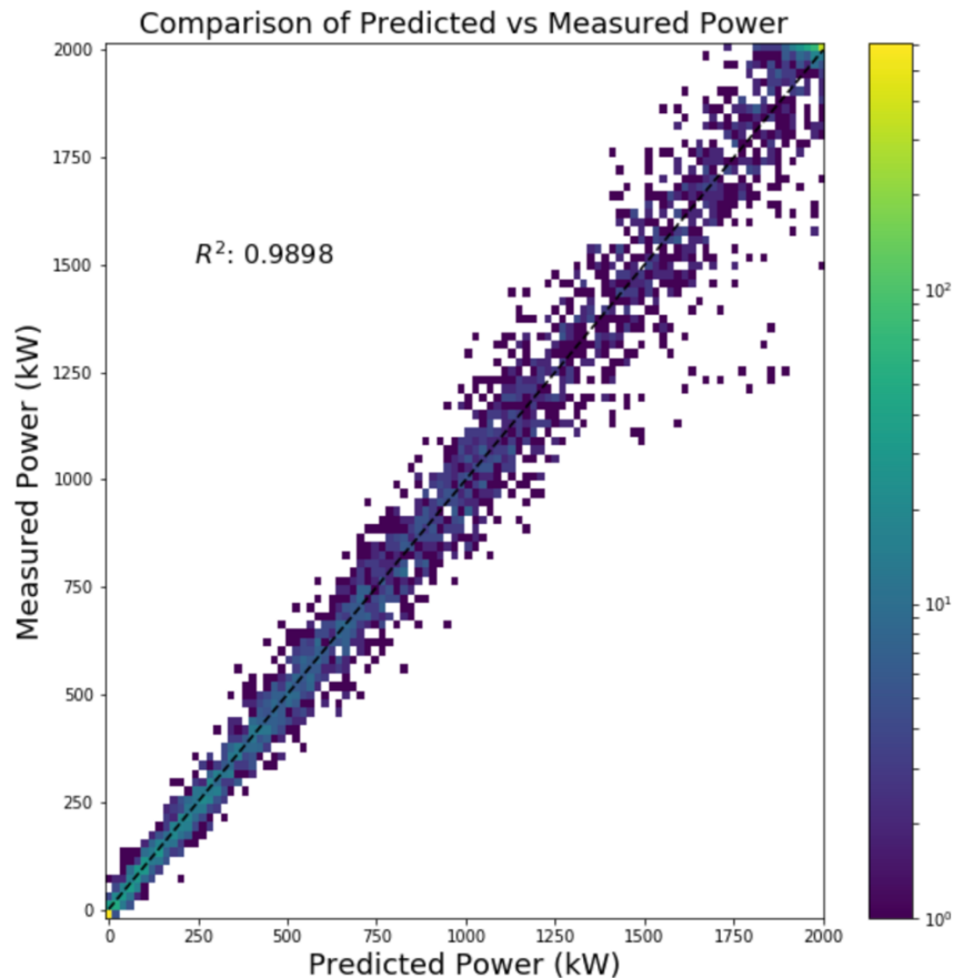
5 Figure 8: Scatter plot of the measured mean power at the Shagaya wind farm compared to the random forest predicted mean, with the black line indicating a linear fit with a R^2 of 0.99.
