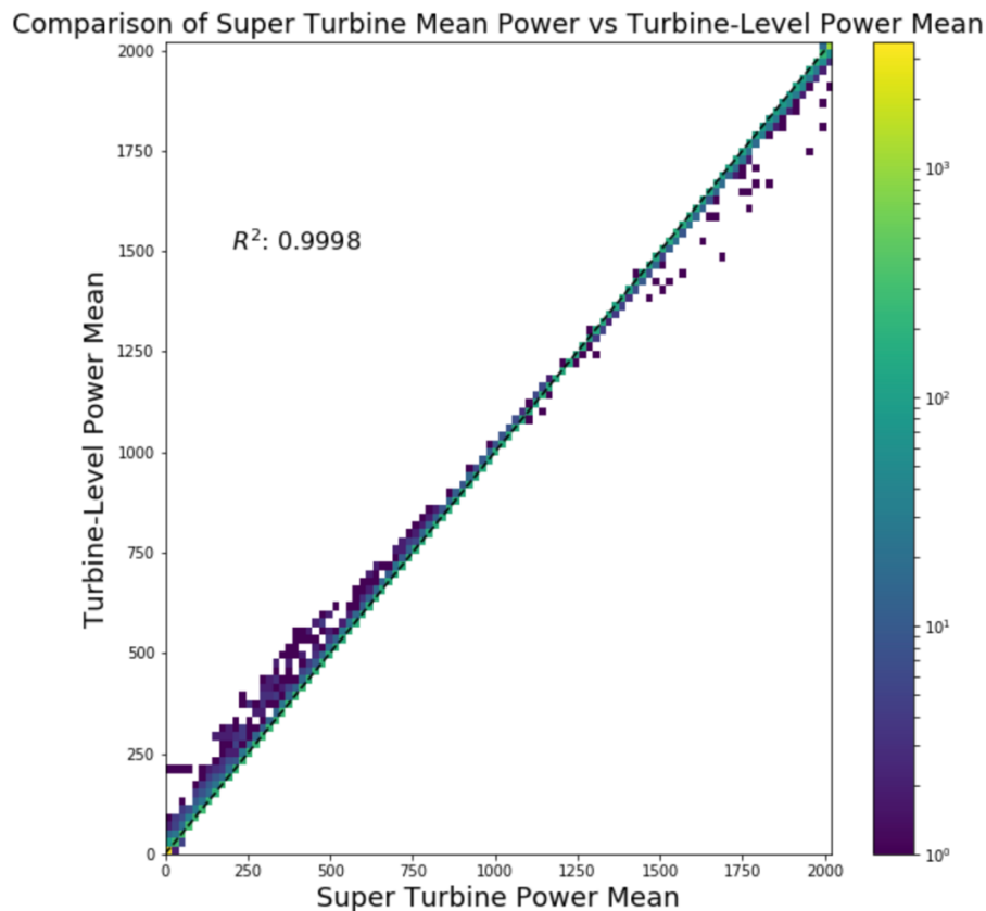
15 Figure 6: Scatterplot of the super-turbine power conversion to the turbine-level power conversion from the mean wind speed and wind speeds at the individual turbines at the Shagaya wind farm.
