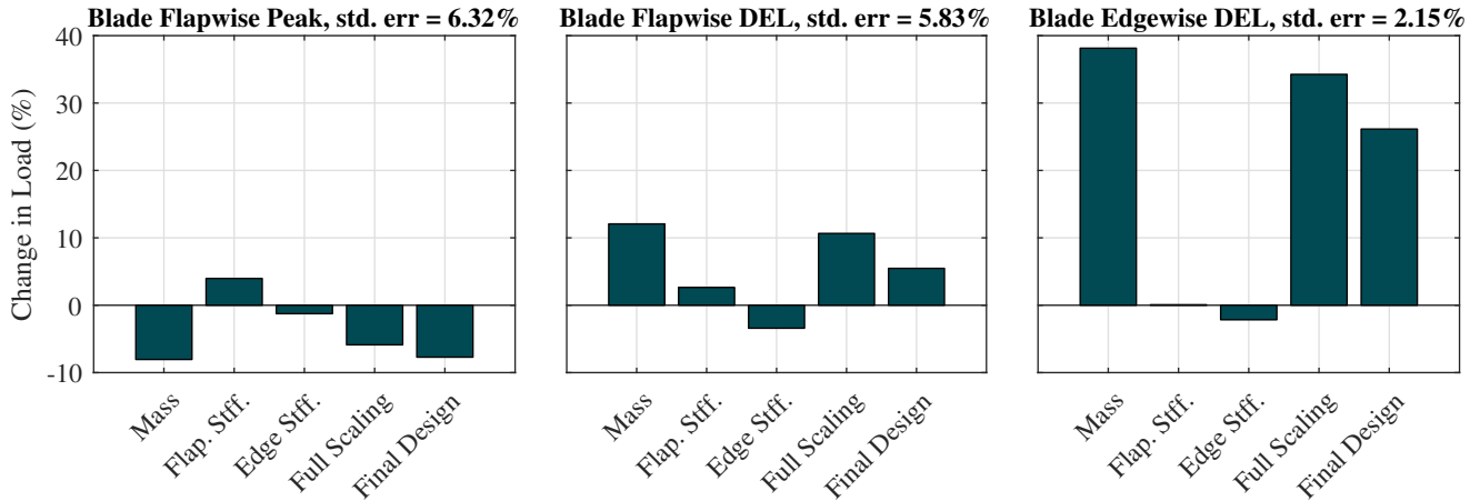
Figure 10. The With \eta = 1.24 and relative to the SUMR-13B with non-scaled structural parameters ( k_M = k_{F_s} = k_{E_s} = 0 , which yield the SUMR-13B loads in Fig. 9), these plots show the effect of mass-independently scaling the mass ( k_M = 1 ), flapwise stiffness sealing ( k_{F_s} = 1 ), and edgewise stiffness sealing ( k_{E_s} = 1 ), and as well as the sealing-combined effect of scaling all of the structural parameters ( k_{\text{All}} = 1 ) on blade loading compared with the non-scaled SUMR-13B ( k_{\text{All}} = 0 Full Scaling, which yield the SUMR-13B loads in Fig. 9 k_M = k_{F_s} = k_{E_s} = 1 ). The standard deviation of error-the residual is computed using the calibration-transformation set in Table 3 and is normalized to the non-scaled SUMR-13B.
