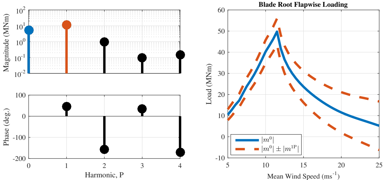
Figure 4. Load harmonic magnitude |m^{zP}| and phase \phi^{zP} for the zeroth through fourth periodic harmonic of the blade root load in the flapwise direction (left) of the SUMR-13A at 25 ms -1 . Mean load (blue) superimposed with the 1P harmonic amplitude (red) with respect to wind speed (right) used to estimate fatigue and extreme loads.
