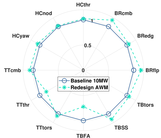
Figure 13. Redesign process including PCM. Left plot: Weibull-averaged ADC. Right plot: ultimate loads. ‘BR’ is blade root, ‘HC’ is hub center, ‘TT’ is tower top and TB is tower base
