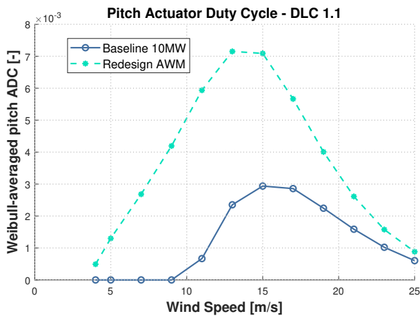
Figure 13. Redesign process including PCM. Left plot: Weibull-averaged ADC. Right plot: ultimate loads. ‘BR’ is blade root, ‘HC’ is hub center, ‘TT’ is tower top and TB is tower base
