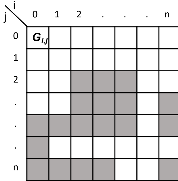
Figure 3. Fictive exclusion zone layer represented as an array: G_{i,j} denotes one mesh point, white and grey squares indicate bad ( G_{i,j} = 0 ) and good ( G_{i,j} = 1 ) locations for a lidar installation respectively, i corresponds to x coordinate or Easting and j corresponds to y coordinate or Northing.
