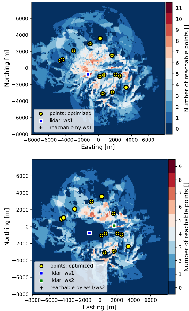
Figure 11. Placing lidars at Italian site: top image - locating first lidar at the combined layer, bottom image - locating second lidar at the second lidar placement layer.
