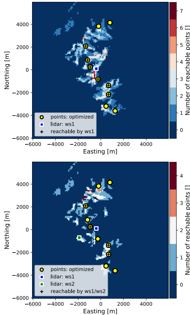
Figure 16. Placing lidars at the Turkish site: top image - locating first lidar at the combined layer, bottom image - locating second lidar at the second lidar placement layer.
