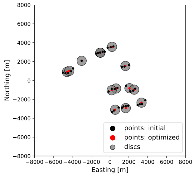
Figure 10. Measurement locations for Italian site: black dots - wind turbine positions, grey circles - discs covering wind turbine positions, red dots - optimized measurement positions (i.e., discs' centers).
