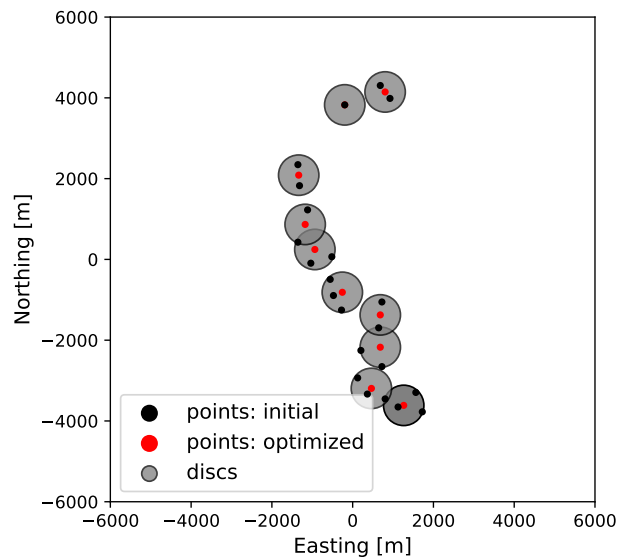
Figure 15. Measurement locations for the Turkish site: black dots - wind turbine positions, grey circles - discs covering wind turbine positions, red dots - optimized measurement positions (i.e., discs' centers).
