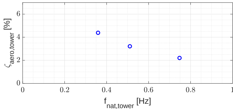
Figure 14. Dependency of aerodynamic damping on tower natural frequency for W = 15 \text{ m/s} .
