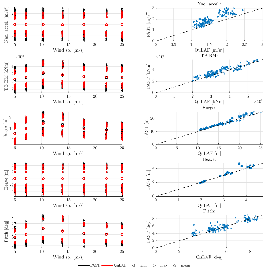
Figure 5. Response to DLC1.6 for FAST and QuLAF. Left: min., max. and mean values for every realisation as function of wind speed. Right: maximum values for FAST as function of the corresponding maximum values in QuLAF
