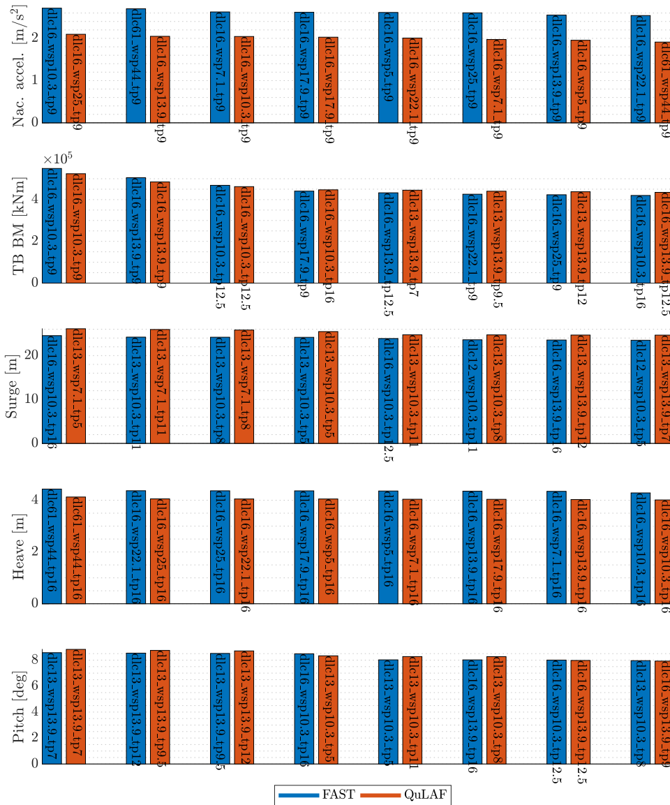
Figure 9. Ranking of the eight highest max. values of each signal and corresponding load case simulations for FAST and QuLAF
