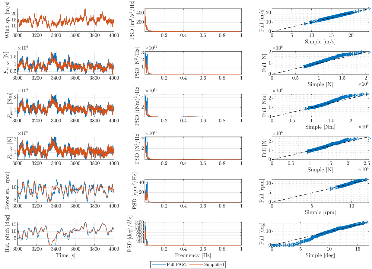
Figure 13. Extracted aerodynamic forcing applied in the surge, pitch and tower deflection degrees of freedom and turbine operational data for DLC1.3 with 13.9 m/s mean wind speed. Left: time series outline. Middle: corresponding power density spectrum (PDF). Right: peak values (sorted) for the full FAST computations as function of the corresponding maximum values in the simplified method.
