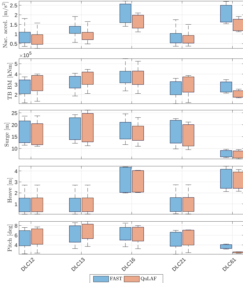
Figure 8. Population of max. values for each of the five load cases
