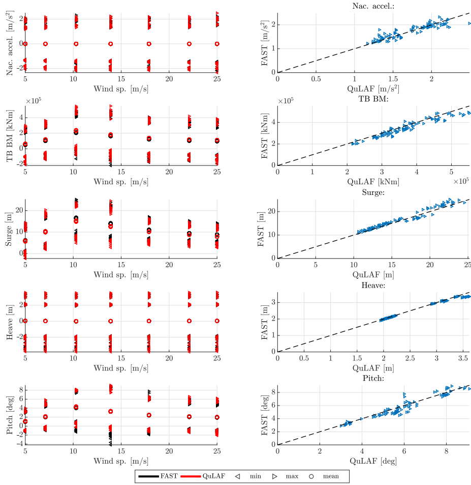
Figure 10. Response to DLC1.6 (without viscous drag) for FAST and QuLAF. Left: min., max. and mean values for every realisation as function of wind speed. Right: maximum values for FAST as function of the corresponding maximum values in QuLAF
