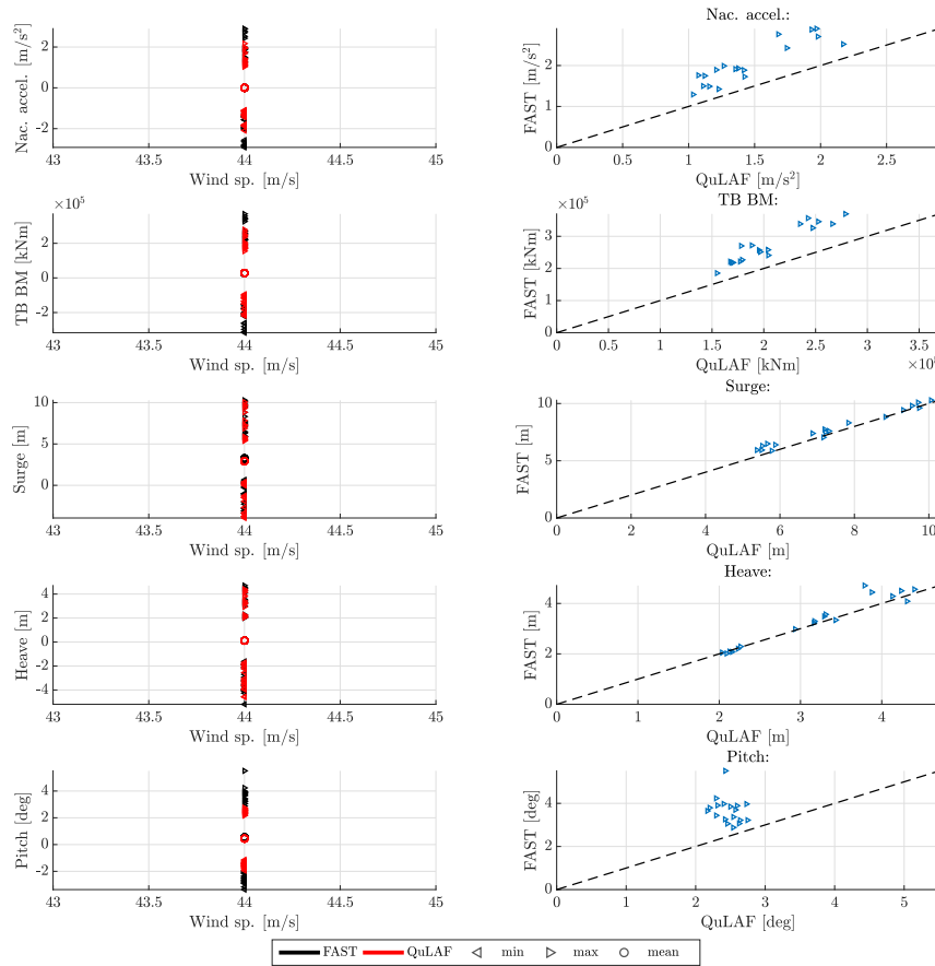
Figure 7. Response to DLC6.1 for FAST and QuLAF. Left: min., max. and mean values for every realisation as function of wind speed. Right: maximum values for FAST as function of the corresponding maximum values in QuLAF
