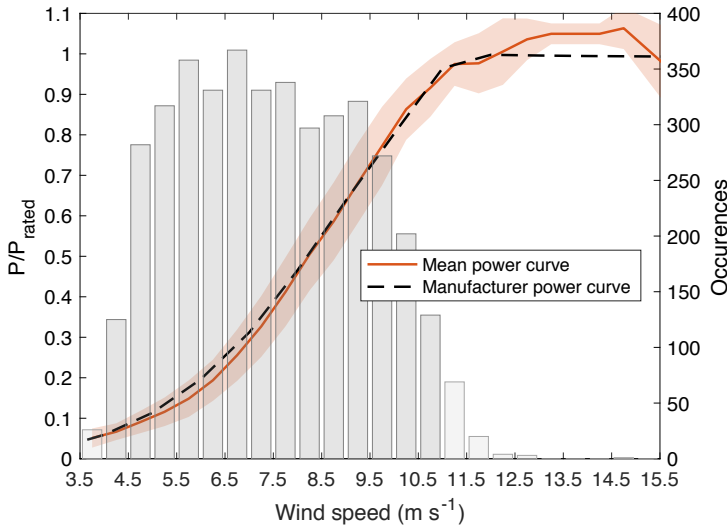
20 Figure 6. Mean power curve for Turbine C based on 80-m lidar wind speed measurements overlaid over the number of power production cases for each 0.5 \text{ m s}^{-1} wind speed bins. The shaded region in the power curve corresponds to \pm 1 standard deviation, and the dark grey histogram corresponds to the wind speed ranges considered in this study.
