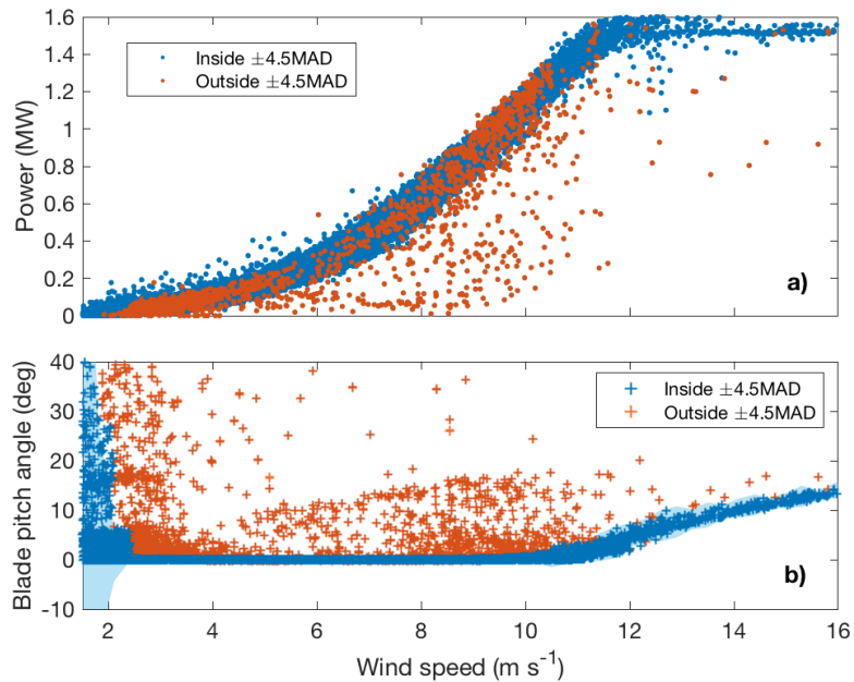
Figure 4. Power curve based on nacelle-measured wind speed (a), and blade pitch angle from a single blade (b) combining data from the four analyzed wind turbines. Red scatter points show 10-min periods filtered out for curtailments, represented by data points outside the MAD envelope. The blue envelope in bottom graph represents \pm 4.5 MAD of the blade pitch angle within 0.5 \text{ m s}^{-1} wind speed bins.
