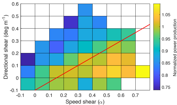
20 Figure 14. Mean normalized power production (turbines A, B, C and D) for all combinations of speed and direction shear that present more than 30 observations. The red line represents the \alpha/\beta threshold.
