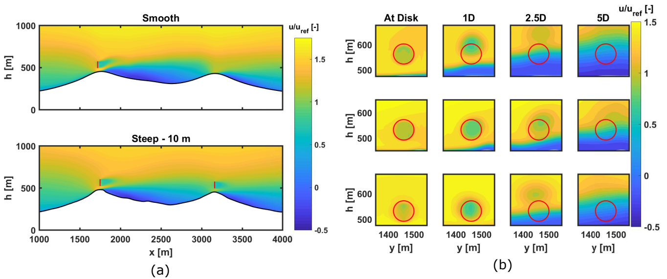
Figure 8. (a) Streamwise velocity profile for smooth and steep terrain, (b) Wake development in the rotor plane at different downstream locations. First row: 1st turbine, steep terrain - 10 m resolution; second row: 2nd turbine, steep terrain - 10 m resolution; third row: 1st turbine, smooth terrain. Rotor position is highlighted by the red circle.
