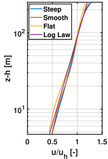
Figure 5. Comparison of normalized mean streamwise velocity at x = 1 .
