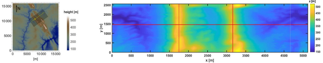
Figure 1. Terrain elevation variation at Perdigão. (Left) Shaded rectangle represents the simulated area, with yellow line passing through the main transect of turbine location (source: (Berg et al., 2017)), (right) shaded region from left figure with intersection of red lines representing the turbine locations.
