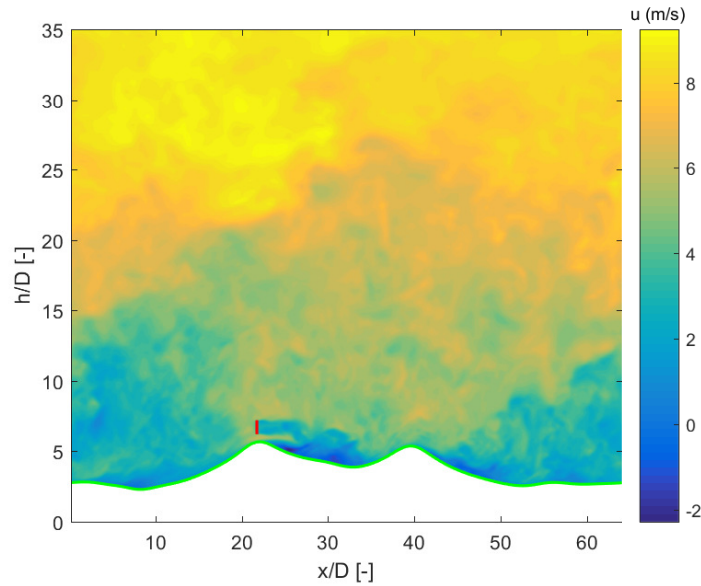
Figure 2. Instantaneous velocity in the streamwise direction along the main transect with turbine (in red).
