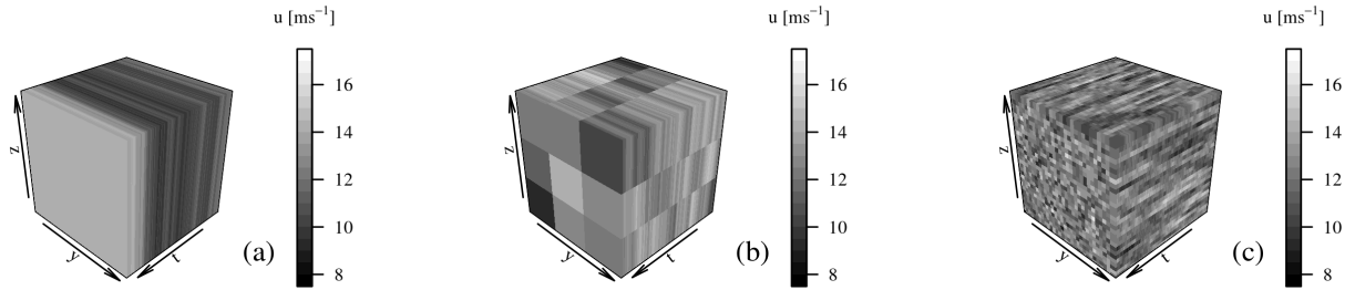
Figure 6. Exemplary visualization of the flow field excerpts for a mean velocity in main flow direction of u = 12.5 \frac{m}{s} . (a) Gaussian type, fully correlated in space. (b) Gaussian type, 3 \times 3 subdivision in space. (c) Gaussian type, delta correlated in space.
