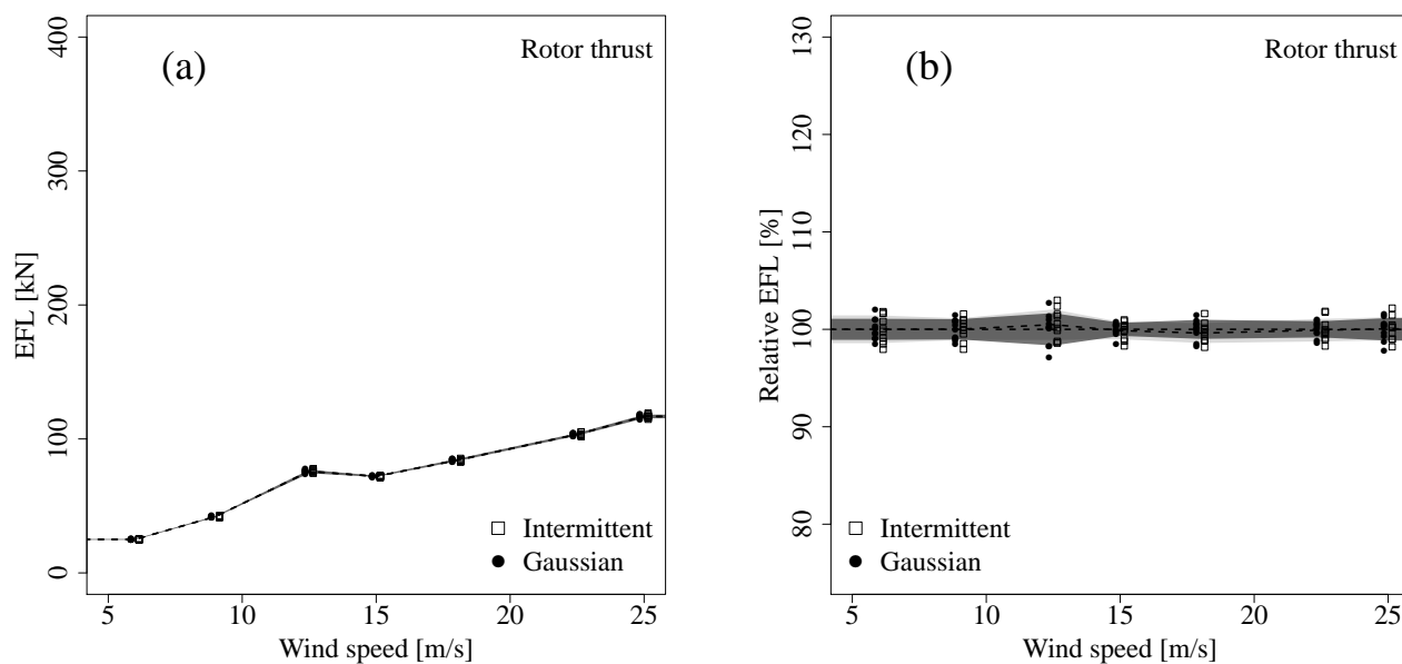
Figure 9. EFL for the rotor thrust for the delta correlated case. Analogous to Fig. 7.
