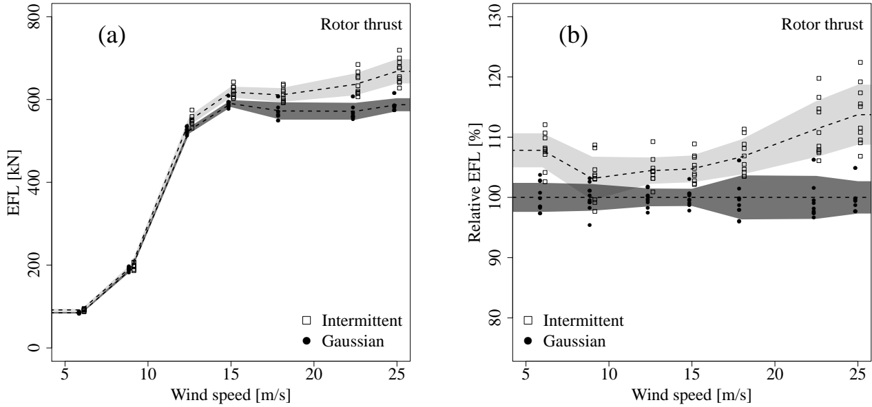
Figure 7. EFL (cf. Eq. (4)) for the rotor thrust for all realizations and all wind speeds for the fully correlated case. The data points were shifted vertically for a better discrimination between intermittent and Gaussian data. The dashed lines represent averages, the shaded area covers \pm one standard deviation around the average. (a) Standard representation. (b) Data normalized with the average of the Gaussian result (Gaussian averages correspond to 100%).
