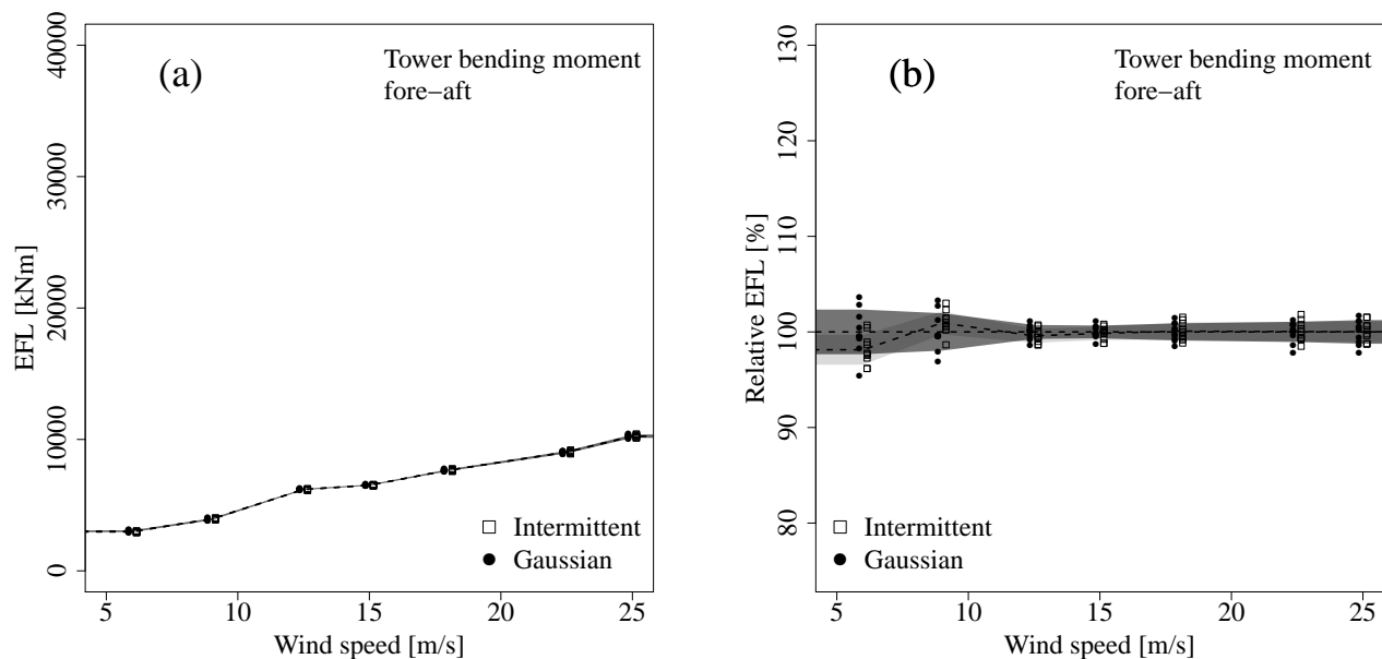
Figure 10. EFL for the Tower base Bending Moment Fore-Aft (TBM FA) for the delta correlated case. Analogous to Fig. 7.
