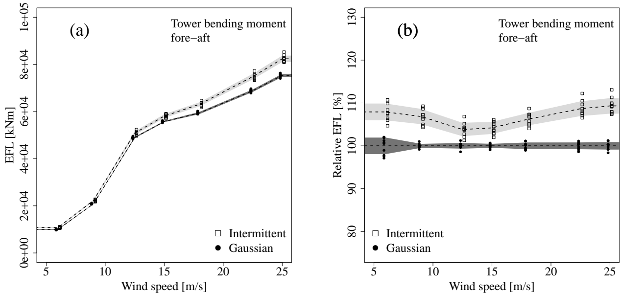
Figure 8. EFL for the Tower base Bending Moment Fore-Aft (TBM FA). Analogous to Fig. 7.
