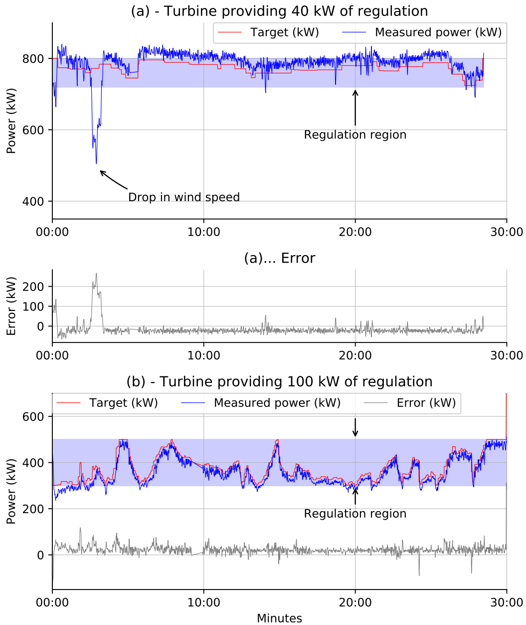
Figure 8. (a) Providing 40 kW of regulation from a single 800 kW wind turbine when operating at rated power. Note that the offset observed is discussed in Section 3.2. (b) Providing 100 kW of regulation. Blue shaded region in (a) & (b) is the range of possible regulation
