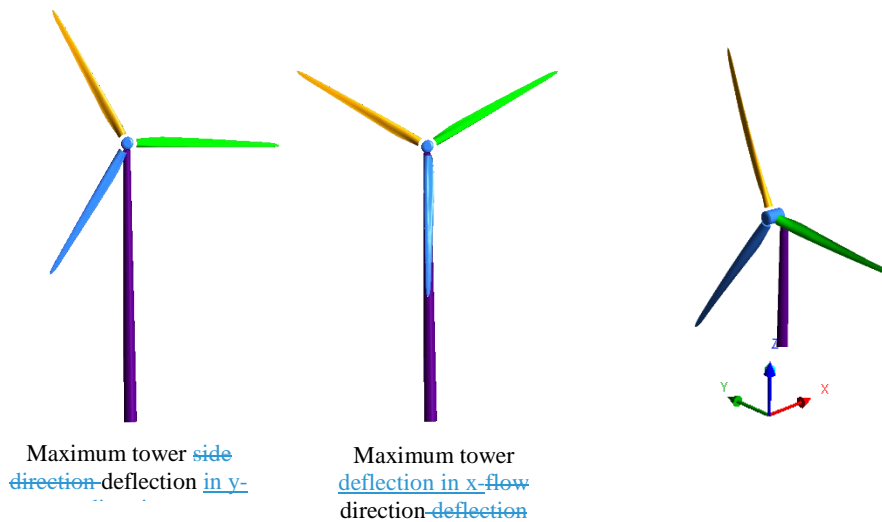
Figure 10. Rotor position for the maximum tower deflections.
