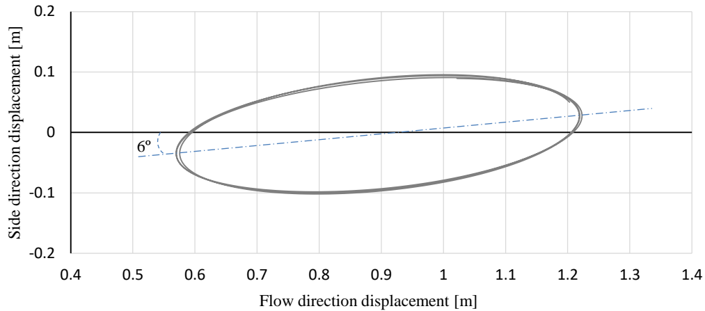
Figure 11. Tower head motion on a 2D plane.
