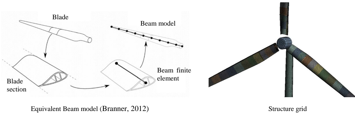
Figure 5. Wind turbine structure.
