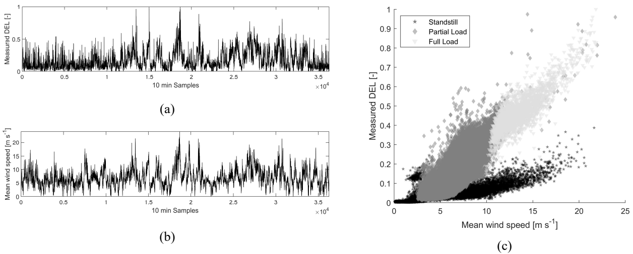
15 Figure 2 – Time series corresponding to (a) normalized measured DELs, (b) mean wind speed and (c) scatterplot of both mean wind speed and measured DELs with a correlation coefficient of 0.74 when data is not filtered by operational modes.
