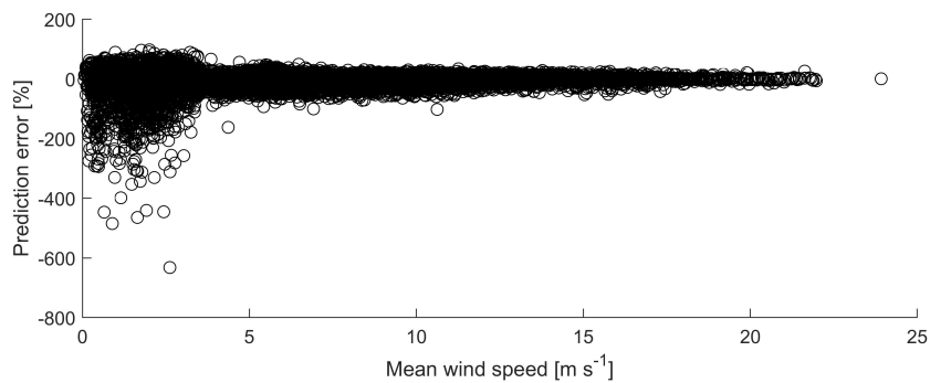
Figure 6 – Wind speed against prediction error
