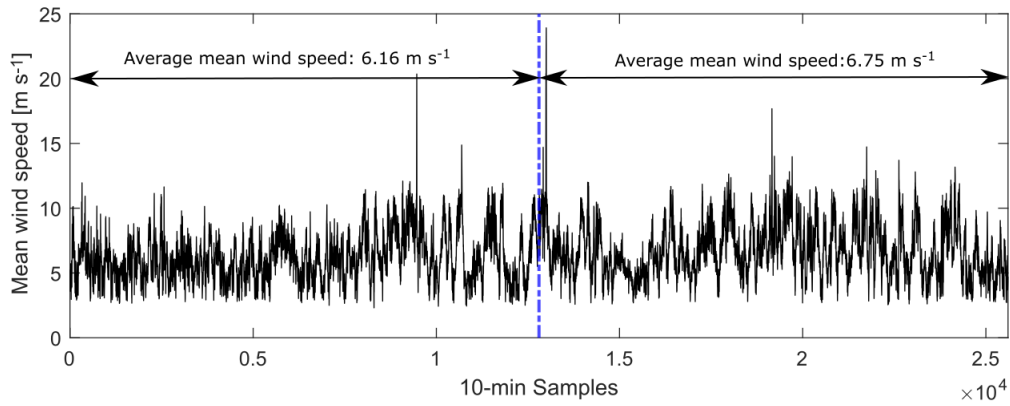
Figure 9 – Mean wind speed during partial load
