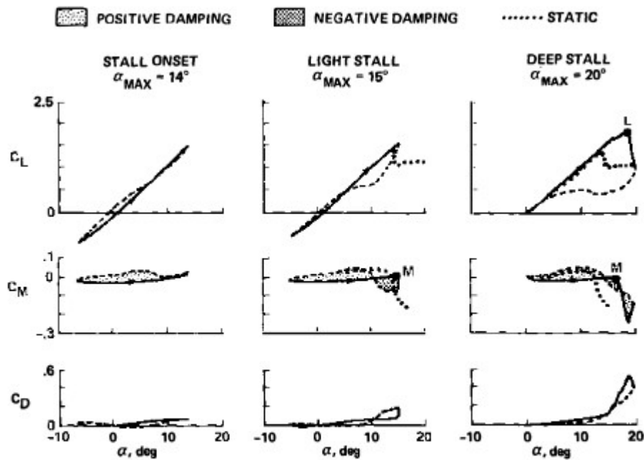
Figure 9 Unsteady forces and moments in three dynamic-stall regimes: M_\infty = 0.3 , \alpha = \alpha_0 + 10^\circ \cos \omega t , k = 0.10 .
