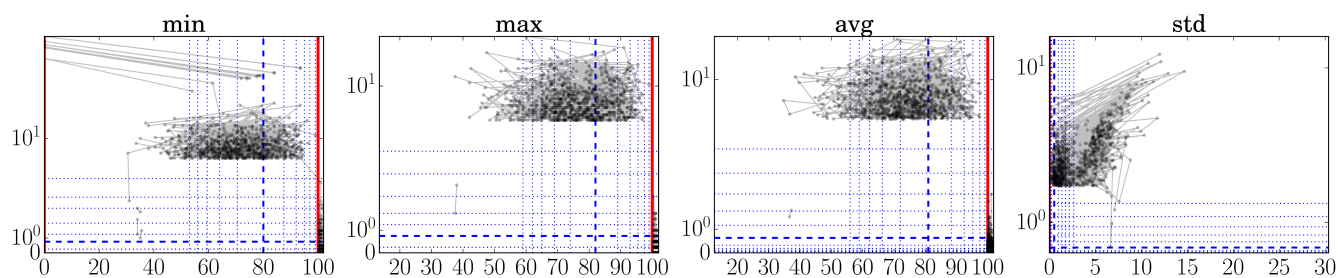
Figure 4. Illustrative plots for visually identifying outliers: MMIJ 21 m relative humidity data [%].
