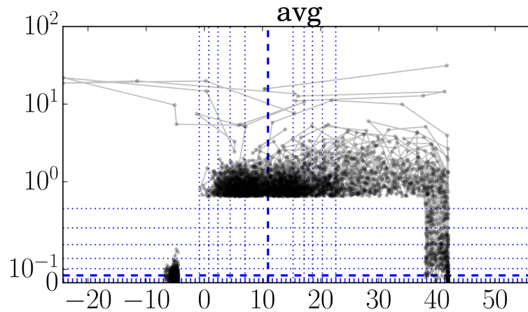
Figure 6. Illustrative plots for visually identifying outliers: FINO 1 72 m ambient temperature data [°C].
