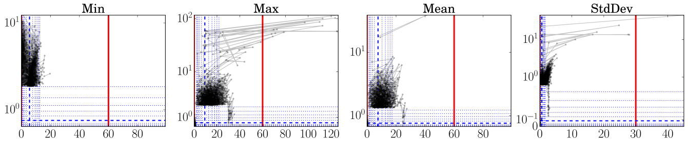
Figure 3. Illustrative plots for visually identifying outliers (cf. pages 8–9 for an explanation): OWEZ 21 m NW ultrasonic anemometer horizontal wind speed data [m/s].
