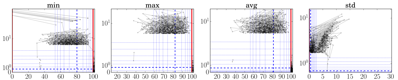
Figure 4. Illustrative plots for visually identifying outliers (cf. pages 8–9 for an explanation): MMIJ 21 m relative humidity data [%].
