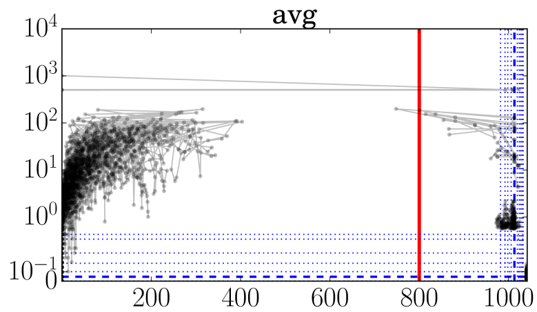
Figure 5. Illustrative plots for visually identifying outliers (cf. pages 8–9 for an explanation): FINO1 21 m air pressure data [hPa].
