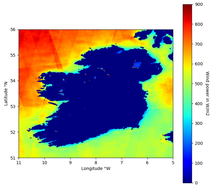
645 Figure 8: Wind power off Ireland over a two-year period running from May 2017 to May 2019 retrieved using the Sentinel-1 SAR Level 2 OCN product. Satellite tracks are visible, particularly in the, northeast. These are an artefact of the analysis.
