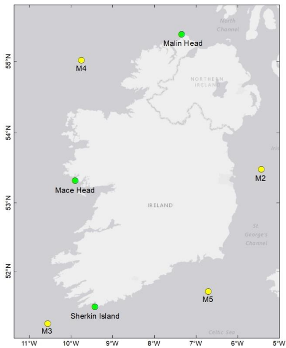
620 Figure 3: Location of metocean buoys (yellow) and coastal weather stations (green) used in the validation of Sentinel-1 SAR surface winds.
