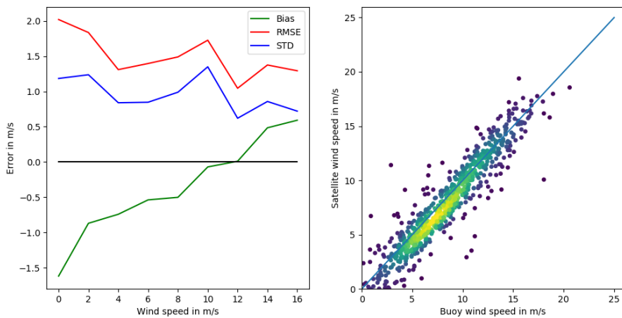
625 Figure 4: Statistical representation of the Sentinel-1 Level 2 OCN error against weather buoy data as a function of SAR wind speeds (left), and scatter plot versus weather buoy data (right).
