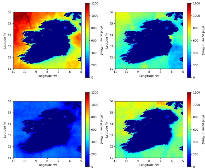
660 Figure 10: Seasonal wind power off Ireland over a two-year period running from May 2017 to May 2019 retrieved using the Sentinel-1 SAR Level 2 OCN product (top left: winter, top right: spring, lower left: summer, lower right: autumn). Satellite tracks are visible, particularly in the, northeast. These are an artefact of the analysis.
