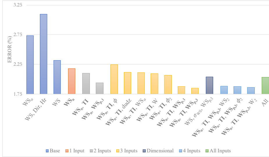
Figure 5. MAPE at Perdigo averaged over all heights. Color coding describes the number of input features used for the ANN. Dark blue bar indicates an additional test for comparison.
