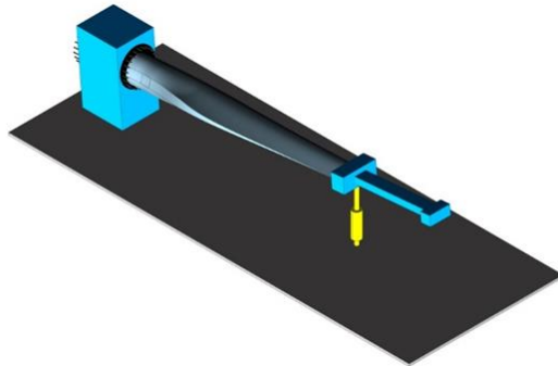
Figure 6. Cantilever structure for root segment test
