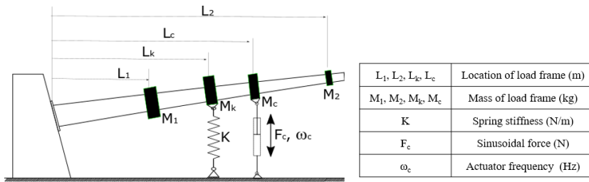
Figure 8. Schematic representation of the root segment fatigue test setup
