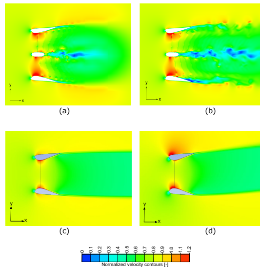
Figure B2. Contours of instantaneous streamwise velocity U_x/U_\infty in the x - y plane for (a) DonQi ® at \alpha = 0 degrees using LB-VLES approach, (b) DonQi ® at \alpha = 7.5 degrees using LB-VLES approach, (c) DonQi ® at \alpha = 0 degrees using 2D URANS approach and (d) DonQi ® at \alpha = 7.5 degrees using 2D URANS approach.
