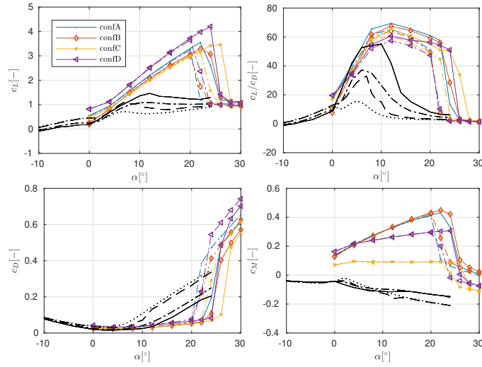
Figure 11. Lift (a), glide ratio (b), drag (b) and pitching moment (d) polar as obtained from CFD for the slat configurations optimized for maximum aerodynamic efficiency using the auxiliary design strategy. The coefficients for the clean (—) and tripped (—.) DU40 profile only, as well as, the clean (—) and tripped (—.) FFA48 base profile only are shown as well.
