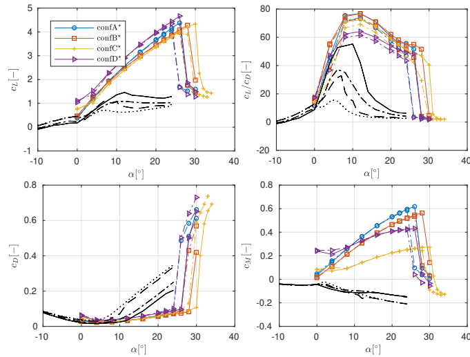
Figure 13. Lift (a), glide ratio (b), drag (b) and pitching moment (d) polar as obtained from CFD for the slat configurations optimized for maximum aerodynamic efficiency using the integral design strategy. The coefficients for the clean (—) and tripped (---) DU40 profile only, as well as, the clean (—) and tripped (---) FFA48 base profile only are shown as well.
