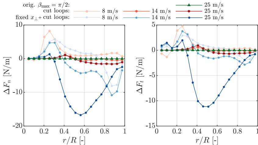
Figure 2. Difference in normal and tangential forces over the NREL 5MW blades at 8, 14 and 25 \text{ms}^{-1} predicted by AL simulations (blades discretized by 19 sections) with different smearing correction speed-up methods with respect to simulations without speed-up.
