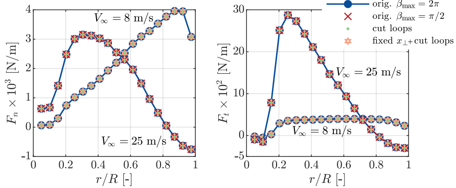
Figure 1. Normal and tangential forces on the NREL 5MW blades at 8 and 25 \text{ms}^{-1} predicted by AL simulations (blades discretized by 19 sections) with smearing correction and different computational speed-up methods. The reference is the original formulation (orig.) with \beta_{\max} = 2\pi .
