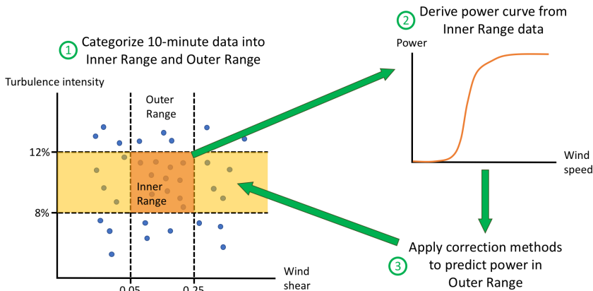
195 Figure 3: How power curves are created and assessed in the Share-3 exercise. The orange and yellow boxes on the left represent the Inner Range, and the Inner Range TI with Outer Range wind shear, respectively.
