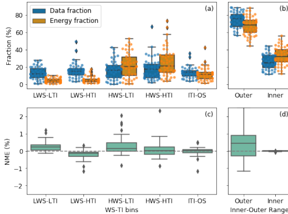
340 Figure 6: (a) Boxplot of data fraction (blue) and energy fraction (orange) in percentage of the submissions across the four WS-TI bins and the ITI-OS bin for the Baseline method. Each colored dot in a bin represents a submission; (b) similar to (a), but for Inner and Outer Ranges. The dots represent the outliers, as in Fig. 5. For each submission, the sum of the fractions of the four WS-TI bins and the ITI-OS bin in (a) equals to the fraction of Outer Range in (b); (c) boxplot of the Baseline's NME in percentage across the same set of WS-TI and ITI-OS bins for the Baseline as in (a). The grey dashed line marks the zero NME, which theoretically is a perfect correction method. The range of NME shown is smaller than the observed, which provides a clearer perspective to contrast different WS-TI bins; (d) similar to (c), but for Inner and Outer Ranges. Similarly, for each submission, the sum of the NMEs in (a) equals to the NME of Outer Range.
