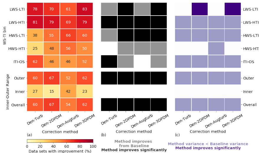
420 Figure 10: (a) Heat map of the four trial methods' improvement fractions upon the Baseline method for the four WS-TI bins and the ITI-OS bin in the Outer Range and the Inner and Outer Ranges, calculated by combining the differences of absolute NMEs from individual submissions. The numbers in each cell annotate the individual improvement percentage; (b) heat map illustrating whether a trial method yields smaller absolute NME than the Baseline on average in each data bin (grey) or not (white), and whether the result is statistically significant after performing the one-sided matched-pair t-test with an alpha of 0.05 (black); (c) heat map 425 representing whether the NME variance of a trial method is smaller than the NME variance of the Baseline method in each data bin (light purple) or not (white), and whether the result is statistically significant after performing the Levene's test with an alpha of 0.05 (dark purple).
