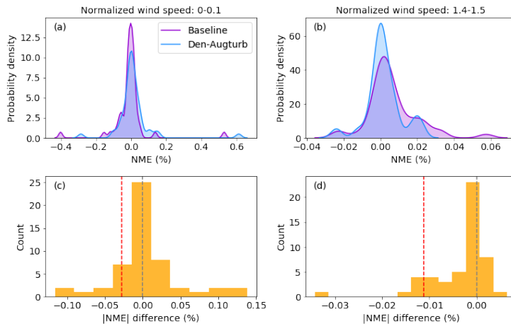
480 Figure 12: (a) Probability density distribution of NME from the Baseline method (purple) and the Den-Augturb method (blue) for 485 the Outer Range normalized wind speeds between 0 and 0.1; (b) as in (a), but for the Outer Range normalized wind speeds between 1.4 and 1.5; (c) histogram of differences of absolute NMEs between the Baseline and the Den-Augturb shown in (a); (d) as in (c), for the differences shown in (b). The grey and red dashed lines denote the zero NME difference and the 10 th percentile of NME differences, respectively. Note that the ranges of the panel axes differ.
