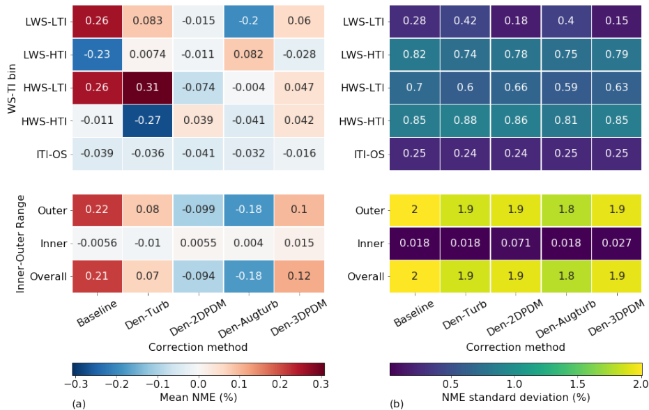
370 Figure 8: (a) Heat map of mean NME based on 48 submissions across the four WS-TI bins and the ITI-OS bin in the Outer Range, along with the Inner and Outer Ranges, for 5 correction methods, where blue is negative and red is positive; (b) heat map of NME standard deviation using 48 submissions across WS-TI and Inner-Outer Range bins and correction methods. The annotated number in each cell represents the mean NME or the NME standard deviation of a specific set of data bin and correction method.
