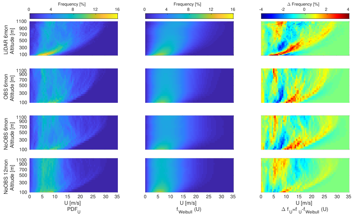
Figure 7. Frequency of occurrence (left), Weibull fit (center) and difference between both (right) of 6 months LiDAR measurements (top row), 6 months OBS model (second row), 6 months NoOBS model (third row) and 12 months NoOBS (bottom row). The entire, (not filtered by LiDAR data availability) was used for the WRF data set.
