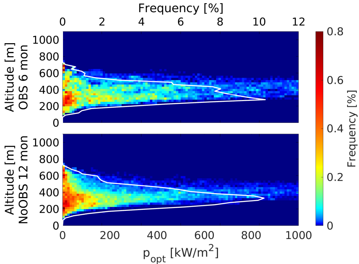
Figure 10. Frequency of optimal traction power over optimal operating altitude based on 6 months OBS (top) and 12 months NoOBS (bottom) assuming a constant tether length of 1500 m. The continuous white line shows the frequency of optimal operating altitude for the whole power range (top abscissa axis).
