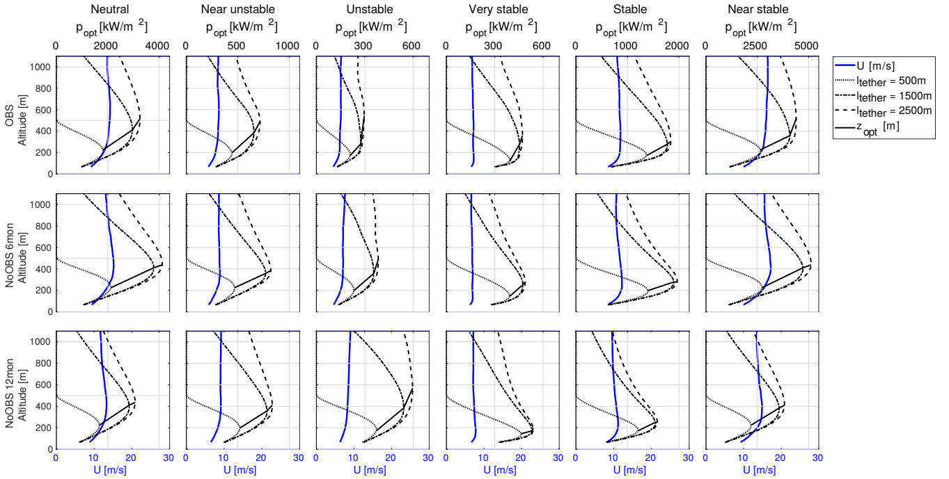
Figure 11. Optimal traction power per wing area p_{opt} (dashed lines) and optimal operational altitude (solid line) estimated based on mean wind speed profiles categorized by Obukhov length ( L ) for 6 months OBS, 6 months NoOBS and 12 months NoOBS simulation with varying tether length ( l_{tether} = 500 - 2500m ).
