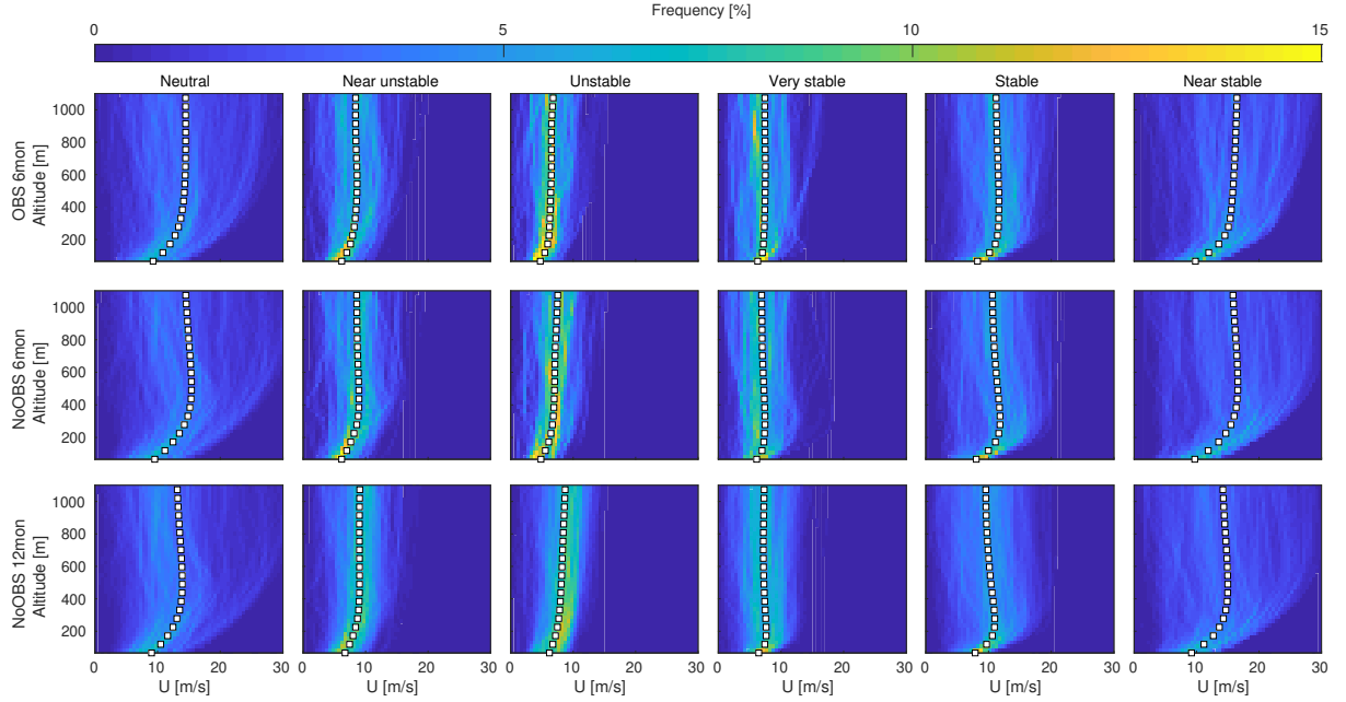
Figure 9. Wind speed U frequency of occurrence and mean (white square) categorized by atmospheric stability according to Obukhov length L (see Table: 1) for 6 months OBS (top), 6 months NoOBS (center) and 12 months NoOBS (bottom).
