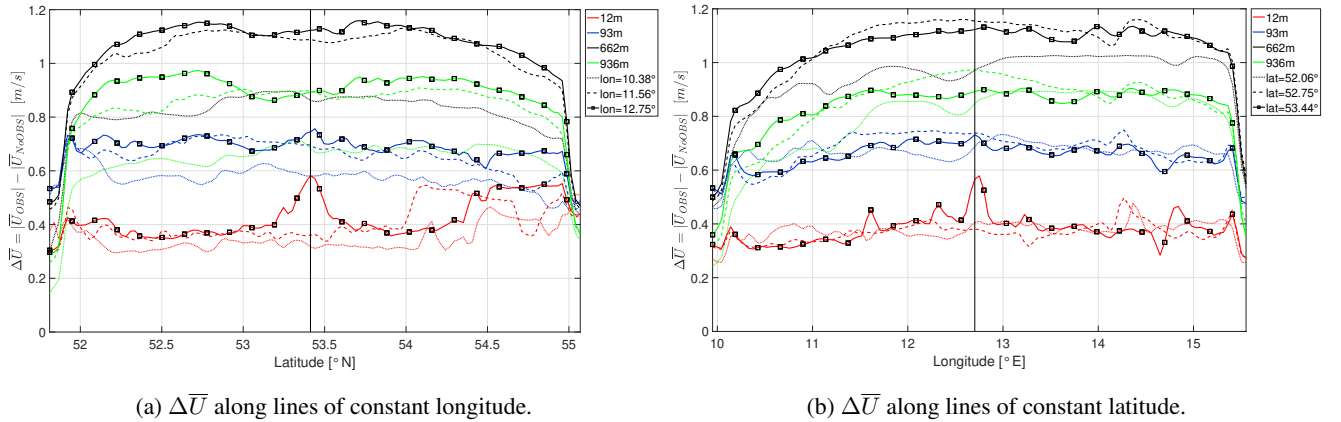
Figure 5. Mean absolute wind speed difference \Delta\bar{U} along lines of constant longitude (a) and latitude (b) within the nudged domain. Approximate distance of d_3 \approx 180\text{km} (dotted lines), d_2 \approx 75 km (dashed lines), d_1 \approx 0 km (solid line) from the center (Lat: 53^\circ 10' 47.00''\text{N} , Lon: 12^\circ 11' 20.98''\text{E} ) Vertical line highlights the grid cell closest to observation.
