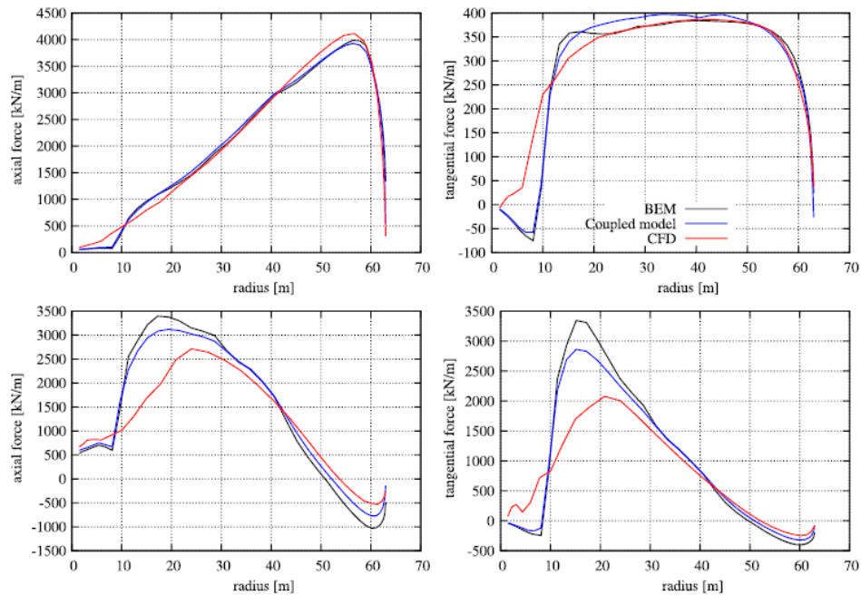
Figure 12. Comparison of axial and tangential forces in normal operation at 8 (top) and 25\text{ m s}^{-1} (bottom) of a blade element momentum (BEM) model, the coupled near and far wake model and full rotor CFD.
