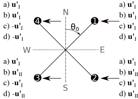
Figure 3. Overview of the assumptions made to determine the cross-contamination values listed in Table 3. In cases with no resonance, the wind vectors u'_{I,II} are identical at the longitudinally separated measurement points. In resonance cases they have an opposite sign. In cases with laterally correlated velocities, the wind vectors at laterally separated measurement points are identical. And in cases with no correlation at points that are laterally separated the wind vectors u'_I and u'_{II} are independent.
