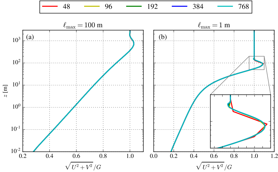
Figure 2. Grid refinement study of the one-dimensional RANS simulation using the limited length scale k - \varepsilon model, for 48, 96, 192, 384 and 768 cells. (a) \ell_{\max} = 100 m. (b) \ell_{\max} = 1 m.
