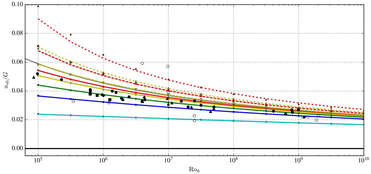
Figure 6. Reproduced from Hess and Garratt (2002). Geostrophic drag coefficient simulated by the limited length scale k - \varepsilon model extended to unstable surface layer stratification, taken at a normalized height of (z+z_0)|f_c|/G = 5 \times 10^{-5} (i.e., in the surface layer), for different Ro_0 , Ro_{\ell} and Ro_{L-} . Black markers represent measurements from Hess and Garratt (2002). Ro_{\ell} = 3.7 \times 10^3 represents \ell_{\max} from Blackadar (1962). Analytic results of Ekman (1905) and Ellison (1956) are summarized in Appendix A
