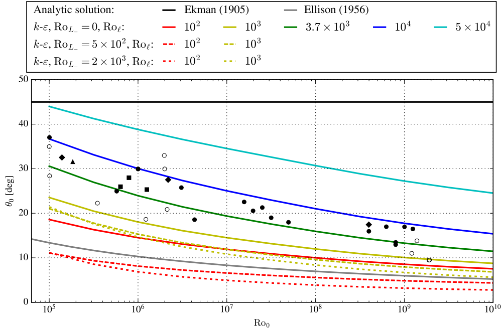
Figure 7. Reproduced from Hess and Garratt (2002). Cross isobar angle simulated by the limited length scale k - \varepsilon model extended to unstable surface layer stratification, taken at a normalized height of (z + z_0)|f_c|/G = 5 \times 10^{-5} for different Ro_0 , Ro_\ell and Ro_{L-} . Black markers represent measurements from Hess and Garratt (2002). Ro_\ell = 3.7 represents \ell_{\max} from Blackadar (1962). Analytic results of Ekman (1905) and Ellison (1956) are summarized in Appendix A.
