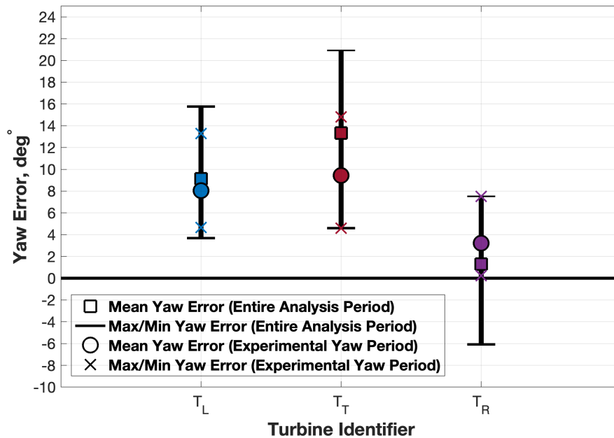
Figure 6. The mean, maximum, and minimum \theta_{err}^V values during the +10^\circ experimental period and the entire DD analysis period.
