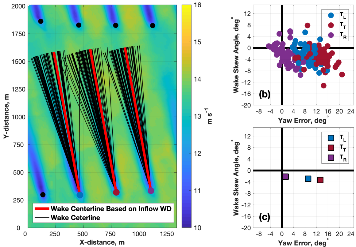
Figure 10. (a). Composite mean TTUKa DD hub-height wind speed ( m s^{-1} ) for the DD analysis period overlaid by the T_L , T_T , and T_R wake centerline from each contributing DD volume (black lines) and the assumed wake centerline based on the DD analysis period mean \theta_{inf}^V value (red lines). (b) The T_L , T_T , and T_R \theta_{skew}^V values plotted as a function of \theta_{err}^V and (c) the turbine-respective mean values from (b).
