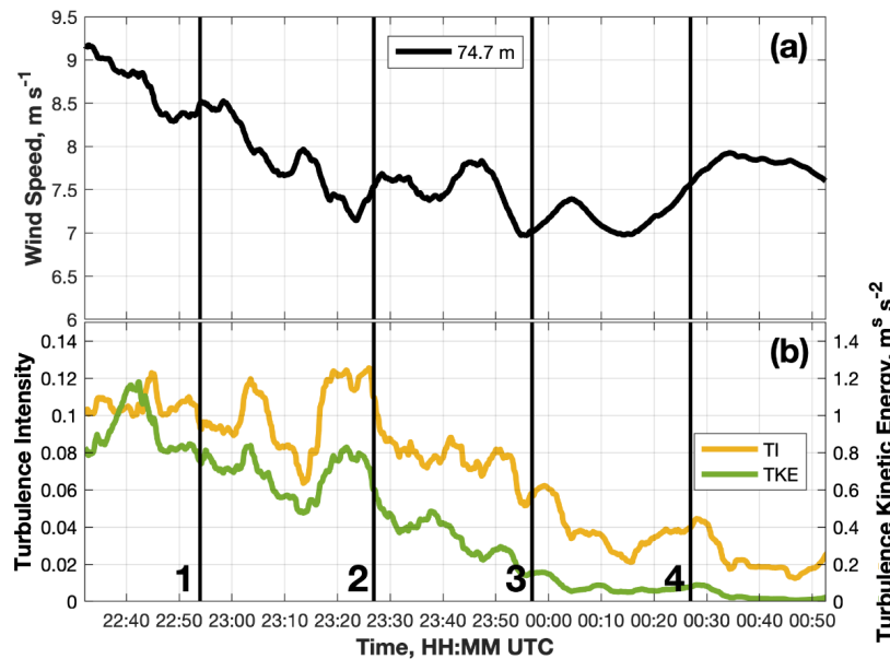
Figure 15. Evolution during the SD data acquisition period of the scan-centric (a) mean wind speed ( \text{m s}^{-1} ) and (b) both TI and TKE at 74.7 m AGL. The scan-centric mean wind speed, TI, and TKE values at the times consistent with the numerically labelled vertical black lines are provided in Table 6.
