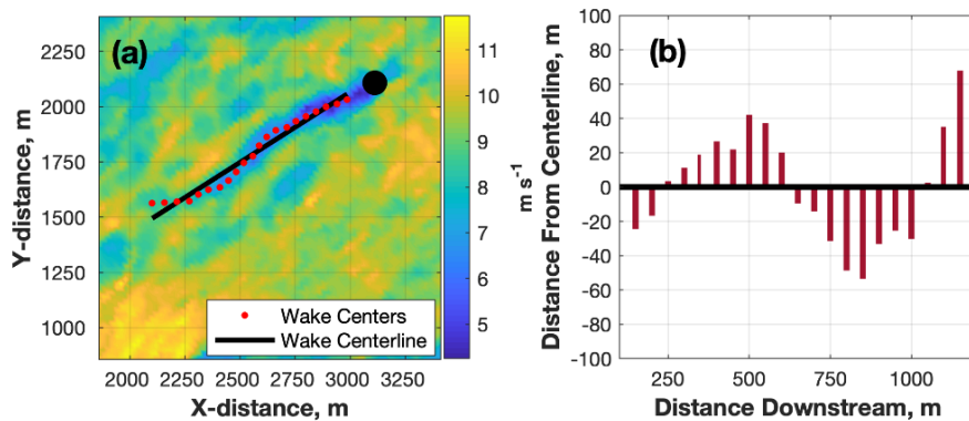
Figure 19. (a) The TTUKa radial velocity wind field ( \text{m s}^{-1} ) at 22:38:25 UTC overlaid by the wind turbine (black circle), the wake centerline (black line), and the individual wake center locations (red circles). (b) Vertical red lines denote the lateral deviation (m) of the wake centers from the wake centerline.
