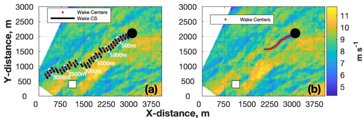
Figure 16. (a) The WTA applied to the TTUKa radial velocity wind field ( \text{m s}^{-1} ) at 22:38:25 UTC overlaid by the location of the instrumented meteorological tower (white square) and the wind turbine (black circle). Also plotted at 100-m intervals are the individual wake cross-sections (black lines) and wake center locations (red circles). (b) Valid wake center locations after applying the wake cessation criteria.
