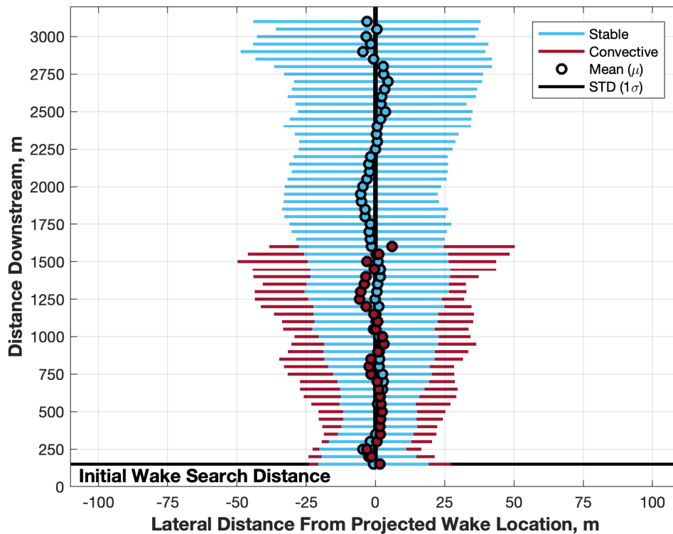
Figure 20. Horizontal wake center meandering mean values (colored circle) and one standard deviation bounds (colored horizontal line) as a function of distance downstream (the plotted colors reflect the ABL stability classification).
