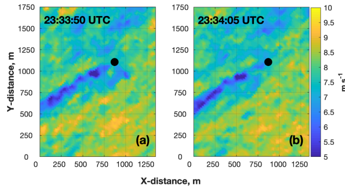
Figure 18. The TTUKa radial velocity wind field ( \text{m s}^{-1} ) at (a) 23:33:50 UTC and (b) 23:34:05 UTC demonstrating wake discontinuities.
