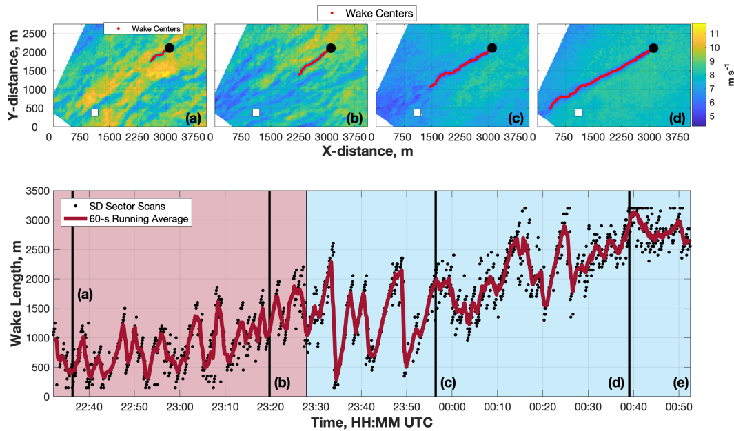
Figure 17. The TTUKa radial velocity wind field ( \text{m s}^{-1} ) at (a) 22:36:21 UTC, (b) 23:19:46 UTC, (c) 23:56:23 UTC, and (d) 00:39:04 UTC overlaid by the location(s) of the instrumented meteorological tower (white square), the wind turbine (black circle), and the WTA-derived wake centers (red circles). (e) Wake length time history overlaid by a 60-s running average of wake length; the red and blue shaded regions denote the convective and stable portions of the SD data acquisition period, respectively.
