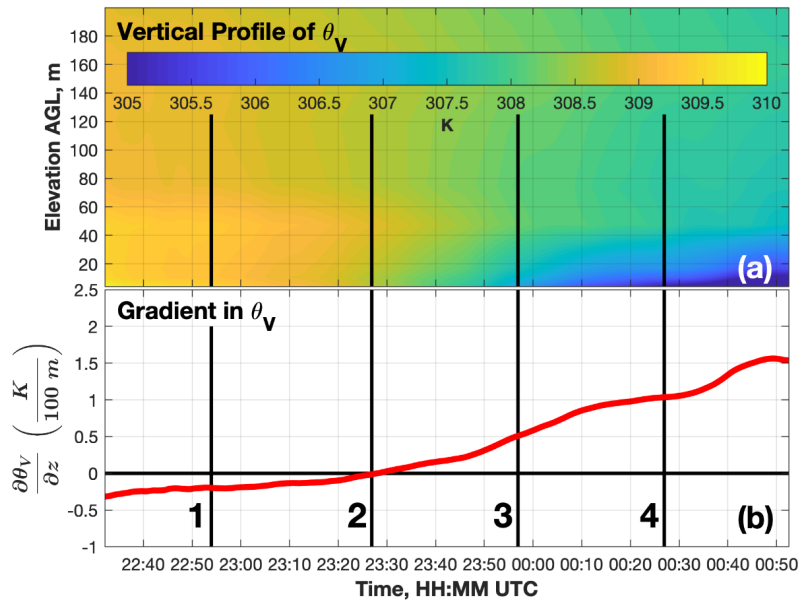
Figure 14. Evolution during the SD data acquisition period of the scan-centric (a) \theta_v vertical profile (K) and (b) the \theta_v gradient (K per 100 m). The magnitude of the \theta_v gradient at the times consistent with the numerically labelled vertical black lines is provide in Table 6.
