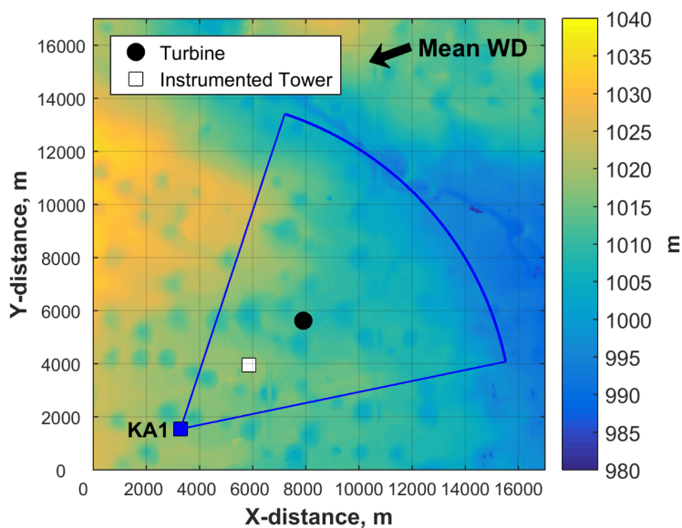
Figure 2. Schematic of the TTUKa SD radar deployment on 12 October 2015. Mapped is the underlying mean sea level elevation (m) overlaid by the location of TTUKa1 (blue square), the radar sector scanned (blue circle arc), the mean wind direction (black arrow), the instrumented meteorological tower (white square), and the wind turbine (black circle).
