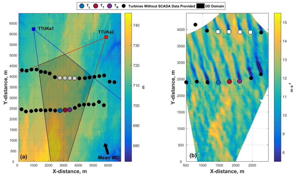
Figure 1. (a) Schematic of the TTUKa DD radar deployment on 14 December 2014 including the radar sectors scanned (red and blue lines), the DD domain (shaded region), the location of individual wind turbines (colored circles [black circles denote turbines whose SCADA data was not provided]), the mean wind direction (black arrow), and the underlying mean sea level elevation (m). (b) TTUKa DD hub-height wind speed ( \text{m s}^{-1} ) at 14:59:29 UTC overlaid by the wind turbine locations.
