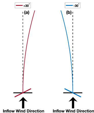
Figure 8. Wake deflection theoretically induced by (a) counterclockwise (i.e. \theta_{\text{err}} = +30^\circ ) and (b) clockwise (i.e. \theta_{\text{err}} = -30^\circ ) yaw rotation relative to a fixed inflow wind direction.
