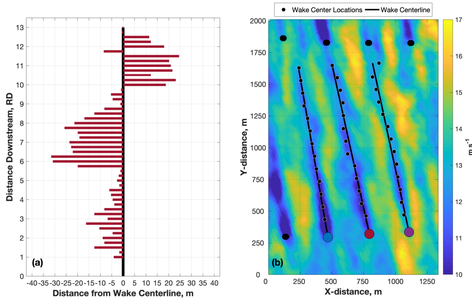
Figure 9. (a) The lateral distance between the T T wake centerline and the wake center locations (i.e. the T T error distribution). (b) TTUKa DD hub-height wind speed (m s -1 ) at 15:30:00 UTC overlaid by the T L , T T , and T R wake centerline and the wake center locations at 1-RD increments.
