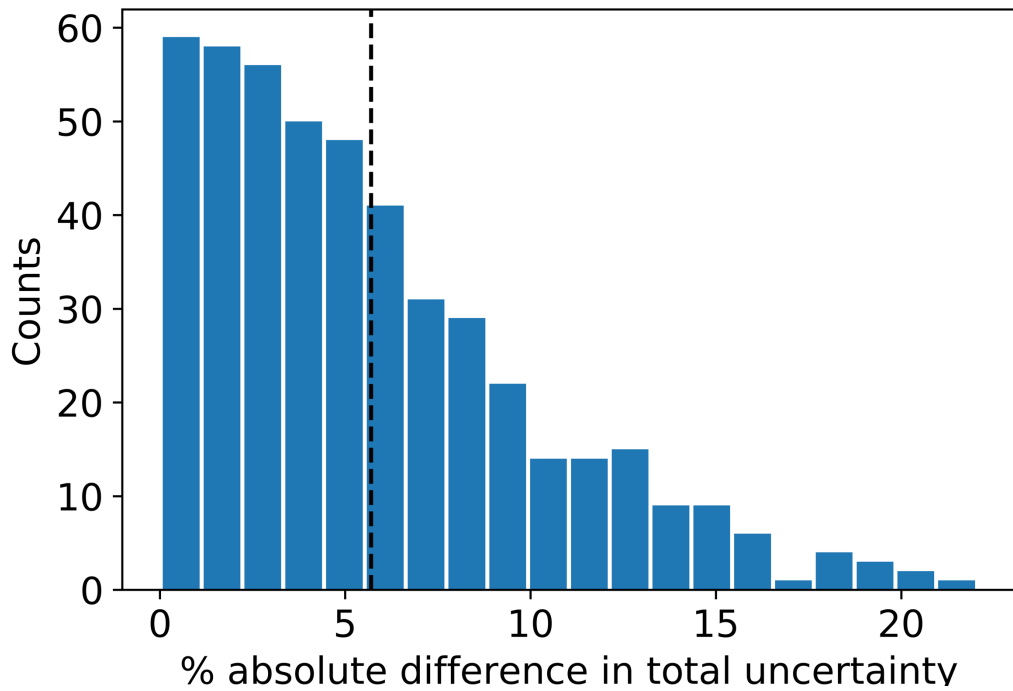
Figure 1: Histogram of absolute percentage differences between the uncertainties calculated using the two different approaches.
