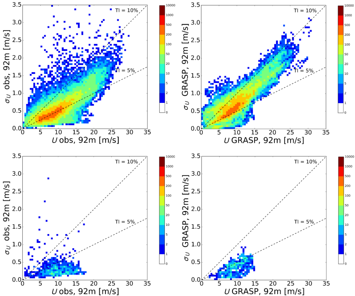
Figure 7 Scatter-density plot of the standard deviation of the wind speed versus the wind speed at the 92-m level. Left panels: observations; right panels: model results, Top panels: entire year; lower panels: only LLJ cases.
