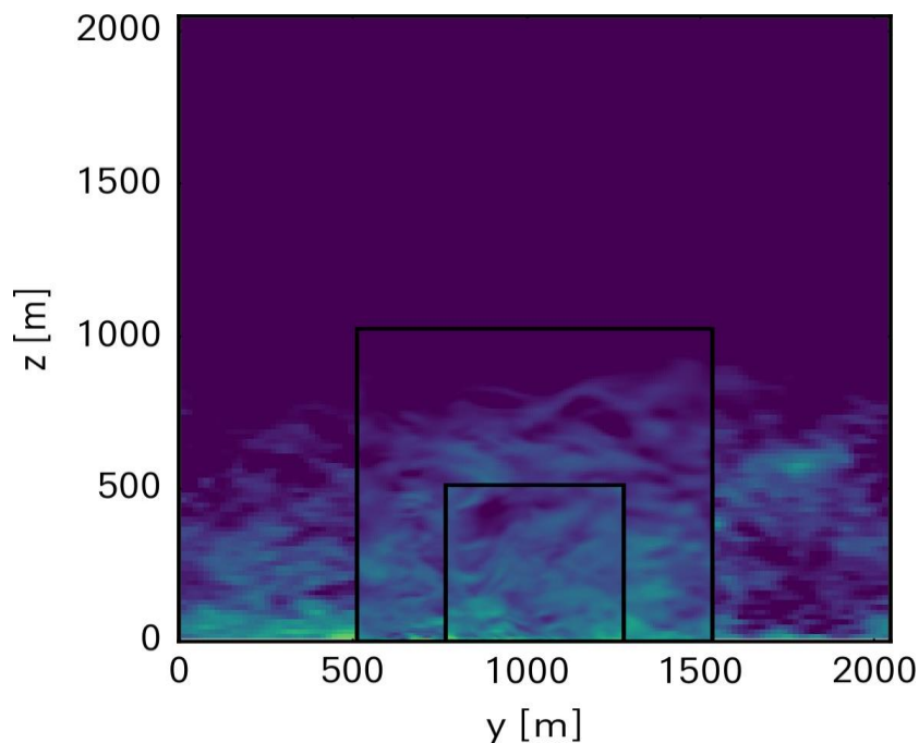
Figure 3 Vertical cross-sections of wind speed in the three different nested LES runs. The coarsest runs use periodic lateral boundary conditions and large-scale forcing from ERA5. The higher resolution runs use lateral boundary conditions from the ‘upper’ nests
