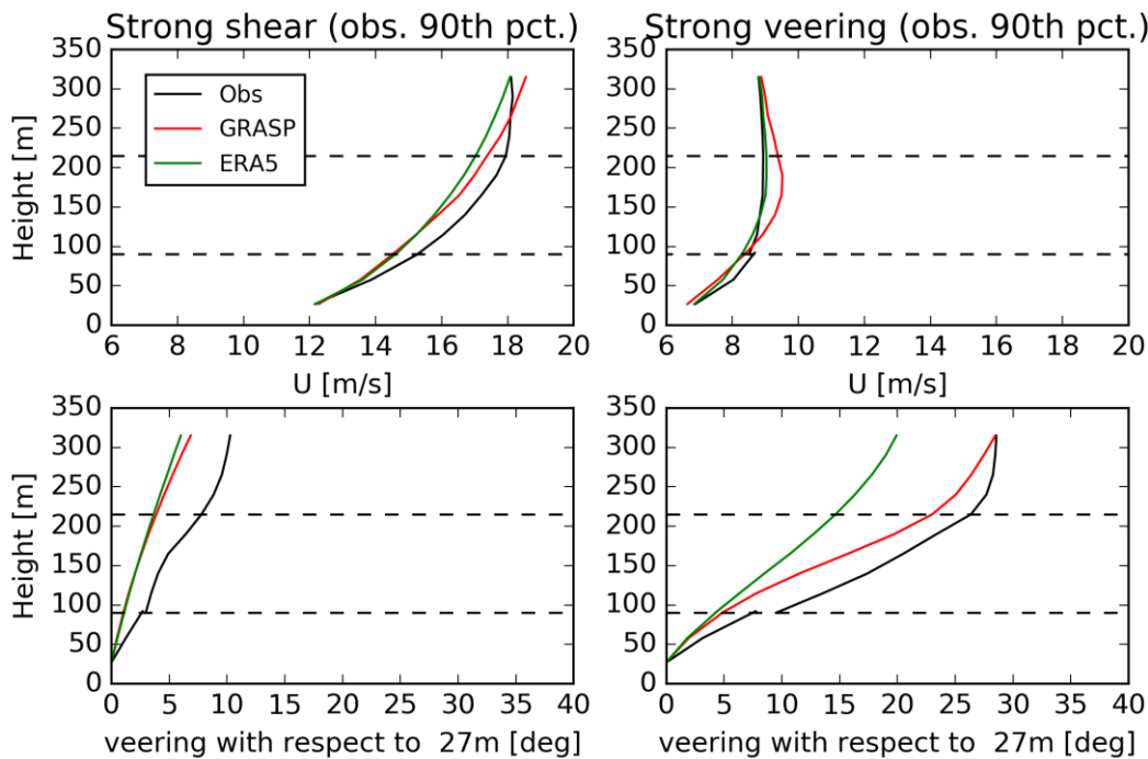
405 Figure 6 Comparison of the 90th percentile strongest shear (left) and veer (right) conditions from observations, ERA5 and GRASP.
