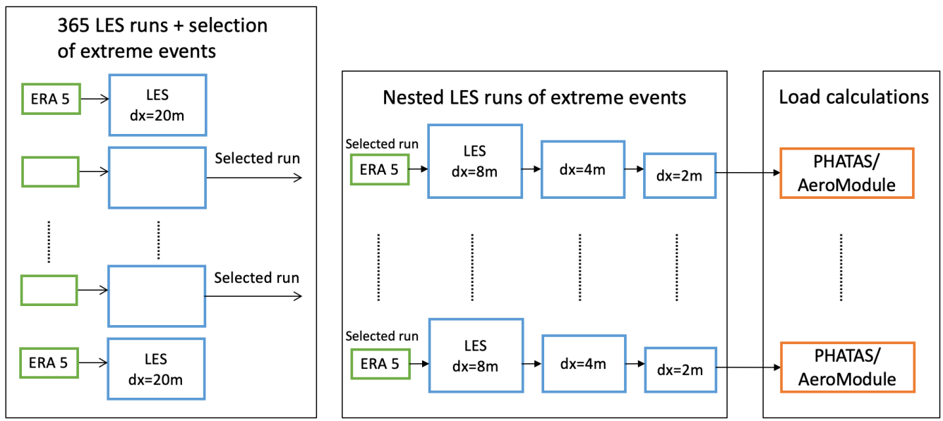
145 Figure 1 Schematic representation of the experimental set-up. From 365 LES runs for a North Sea location, 5 extreme events are selected. These are re-run on higher resolution and the output passed to the aero-elastic models PHATAS and AeroModule.
