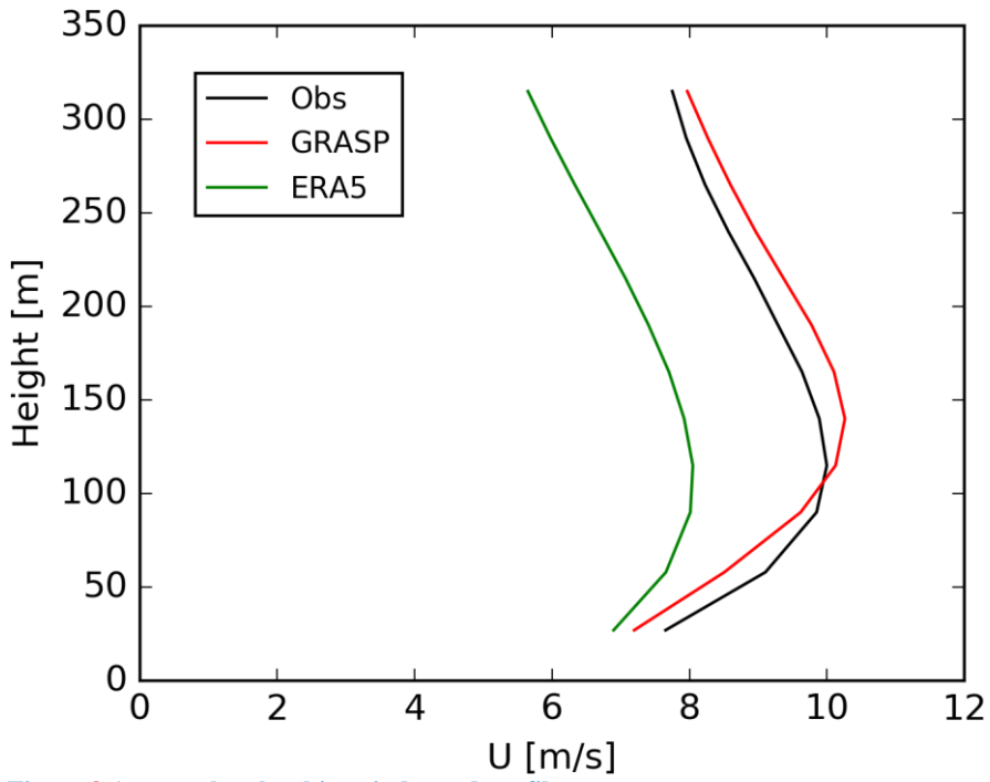
Figure 8 Average low-level jet wind speed profiles.
