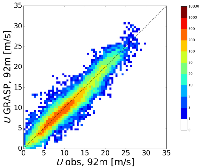
210 Figure 2: Scatter density plot of modeled versus observed 92-m wind speed.
