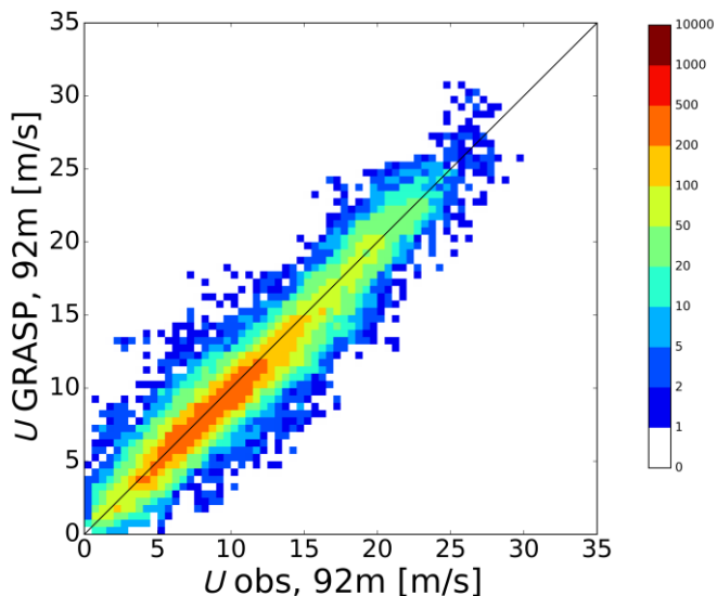
315 Figure 4 Scatter-density plot of modeled versus observed 92-m wind speed.
