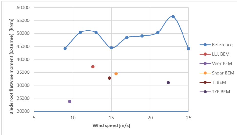
300 Figure 8: Equivalent blade root flatwise moment: DLC1.2 versus GRASP extreme wind events
