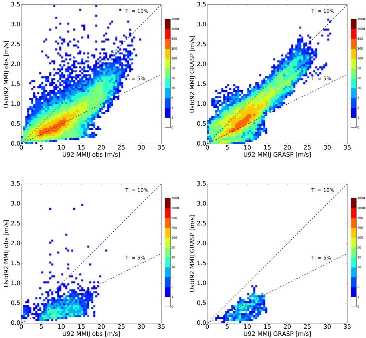
Figure 6 : Scatter-density plot of the standard deviation of the wind speed versus the wind speed at the 92-m level. Left panels: observations; right panels: model results, Top panels: entire year; lower panels: only LLJ cases.
