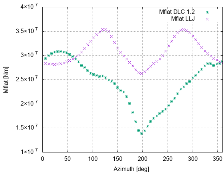
Figure 10 Azimuthally binned averaged flatwise moment: LLJ versus DLC1.2
