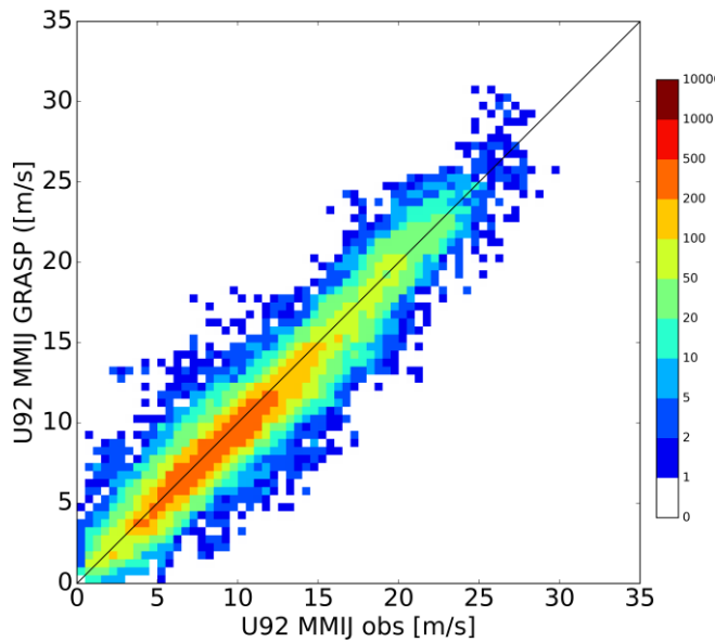
Figure 2: Scatter-density plot of modeled versus observed 92-m wind speed.
