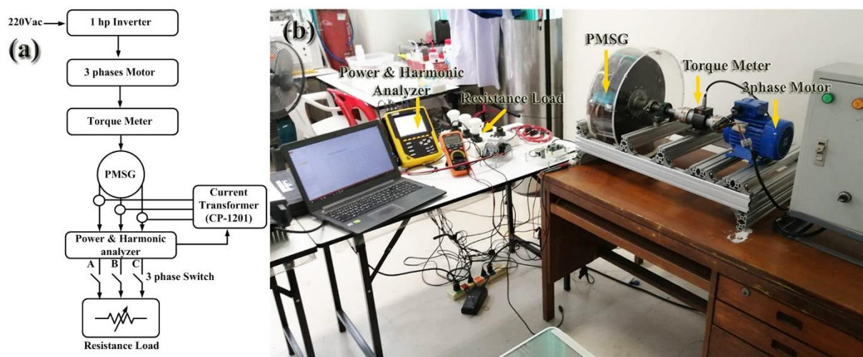
Figure 2: (a) Diagram showing the measurement of the Permanent Magnet Synchronous Generator (PMSG) connected to the motor driver and electrical load; (b) the PMSG experimental testing station.
