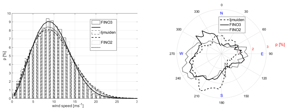
Figure 3. Wind speed (left) and wind direction (right) distributions for the three 24-month datasets from the FINO3, Ijmuiden and FINO2 offshore met mast sites. Derived statistics are summarized in Table 1.
