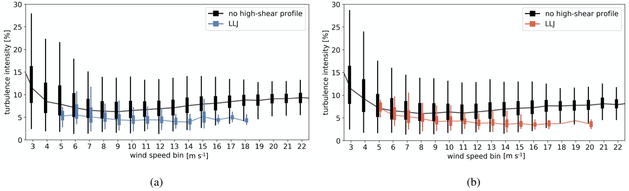
Figure 13. Hub-height ( z = 100 m) distribution of turbulence intensity for wind speed bins between 3 and 22 m s -1 for the NE (a) and SW (b) buoys. Distributions are shown separately for all 10-min periods without a high-shear profile (black) and those with a LLJ profile (colored). Only wind speed bins with at least 10 LLJ profiles are shown. Monotonic shear periods are excluded here for clarity.
