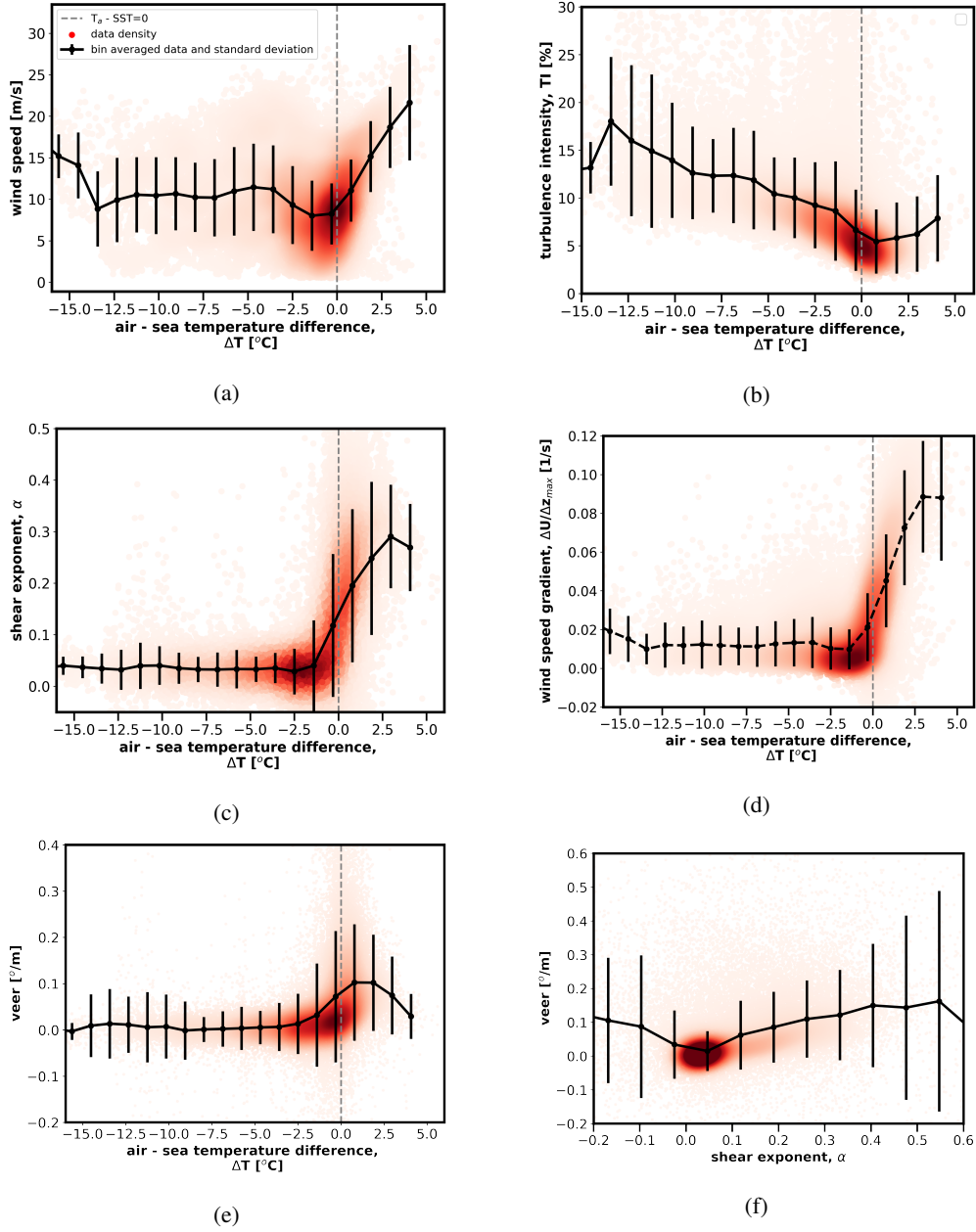
Figure 9. Wind characteristics as they depend on the air-sea temperature difference. Only NE buoy (Table 1) data are shown here. a) Wind speed, b) turbulence intensity, c) wind shear exponent, d) maximum wind speed gradient across the nominal rotor defined here (between 40 m and 160 m), and e) wind veer. A relationship between the wind shear exponent and wind veer is provided in subfigure f.
