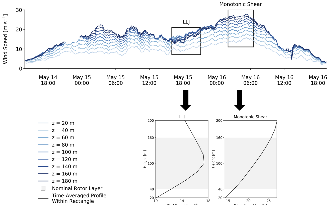
Figure 2. Example of high-shear event as measured by lidar on the NE buoy. Location of the NE buoy is provided in Table 1. Time series between May 14, 2020, 13:50 UTC and May 16, 2020, 19:30 UTC (top). The data within the two black boxes are time-averaged and shown below the time series as examples of low-level jet (LLJ) and monotonic-shear periods.
