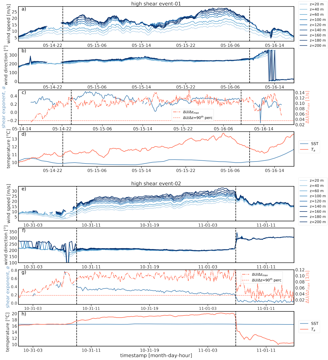
Figure 8. Two examples of high-shear events measured at the NE buoy (Table 1) in year 2019. Subfigures show time series of wind speed (a, e), wind direction (b, f), wind shear (power-law exponent \alpha ), and wind speed gradient ( \Delta U/\Delta z_{max} ) (c, g), and air ( T_a ) and sea-surface temperature (SST) (d, h). Vertical dashed lines represent the start and end times of the high shear events. First example is shown with subfigures a, b, c, d, and second example is shown in subfigures e, f, g, h.
