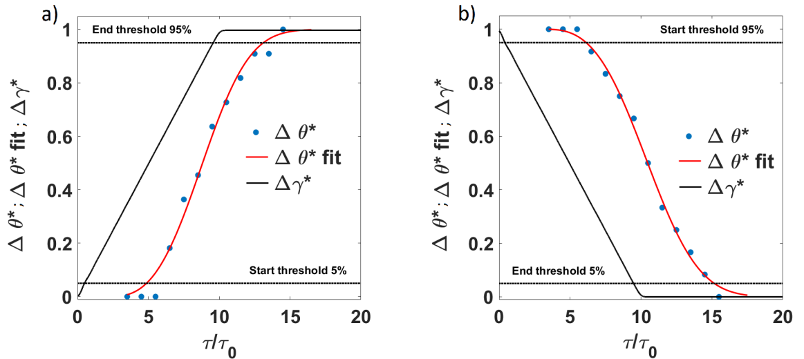
Figure 6. Example of cycle-averaged wake deviation history during yaw manoeuvre for configuration HIT1 P1. Positive yaw variation (a) and negative yaw variation (b). Symbols: —, ●, — fitted, - - start thresholds. Data fitted for \tau > \tau_{lag} .
