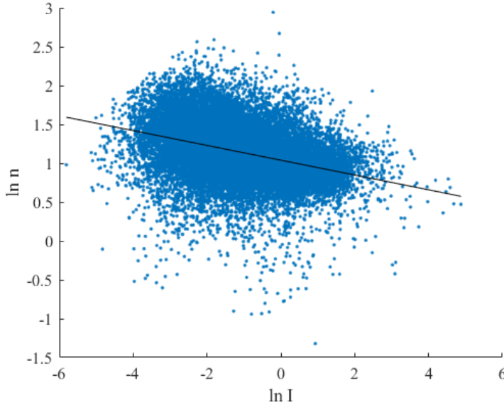
Figure 8: Evaluation of Eq. (7) to derive the constants N and q .
