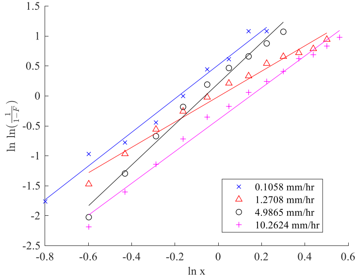
195 Figure 6: Evaluation of Eq. (4) for precipitation intensities 0.1058, 1.2708, 4.9865 and 10.2624 mm/hr.
