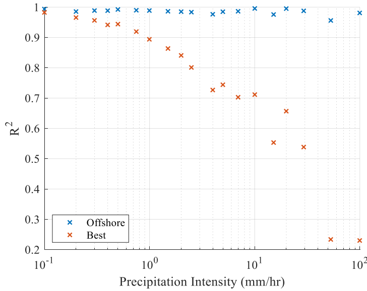
255 Figure 11: Coefficient of determination of the offshore DSD and the Best DSD across a range of precipitation intensities.
