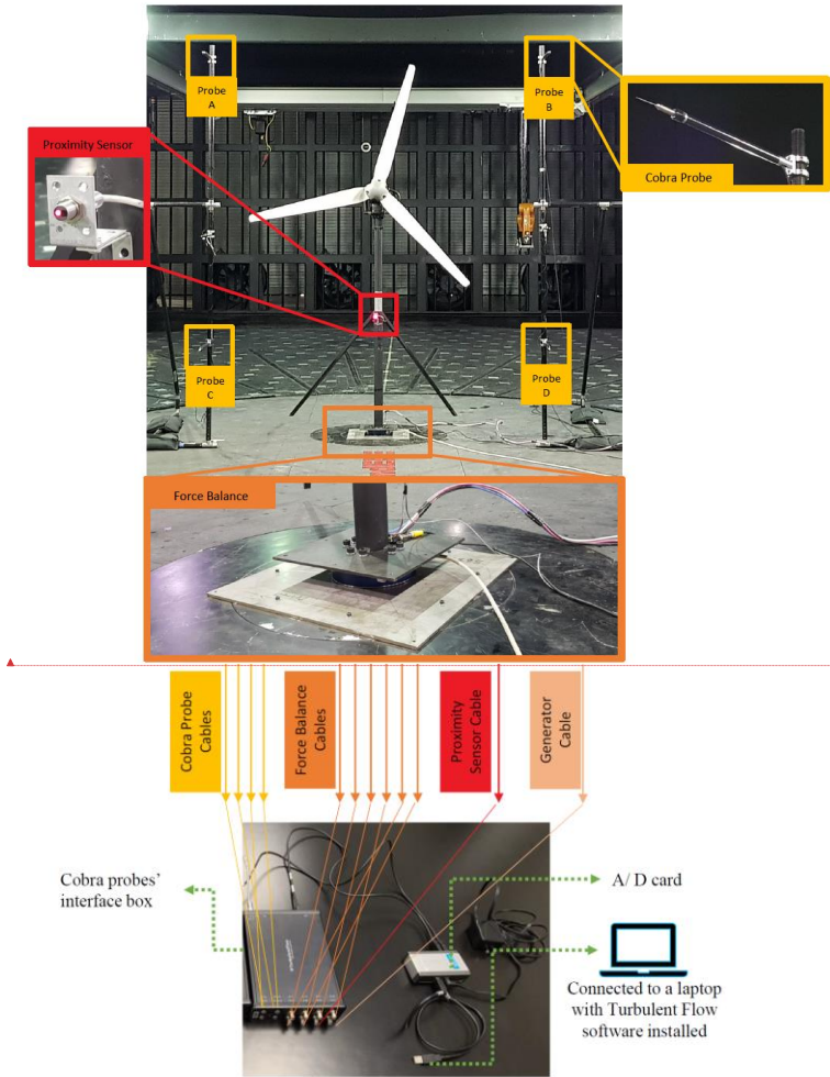
FigureFig. 3.3: Setup for measuring power performance and dynamic loads for different types of inflow
