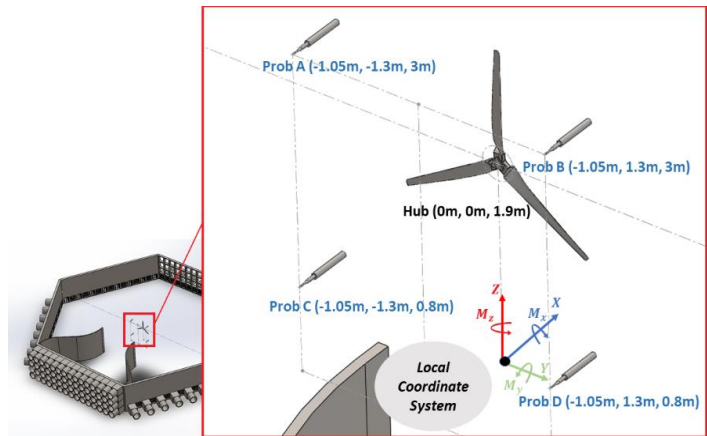
FigureFig. 4.4: The arrangement of cobra probes and HAWT relative to local coordinate system
