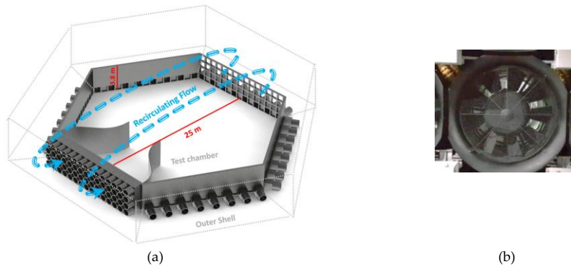
Figure 2: (a) the test chamber and the contraction walls with the flow recirculation path through the outer shell in closed circuit 2D flow mode, (b) the adjustable vanes at the inlets of the 60 fans at 70% opening vanes state
