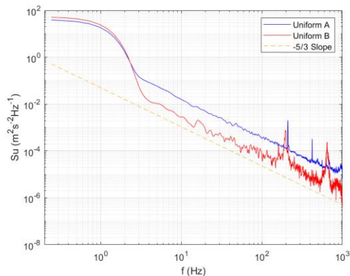
FigureFig. 5.5: Comparison of turbulent velocity spectra for the 5 m/s uniform flow cases
