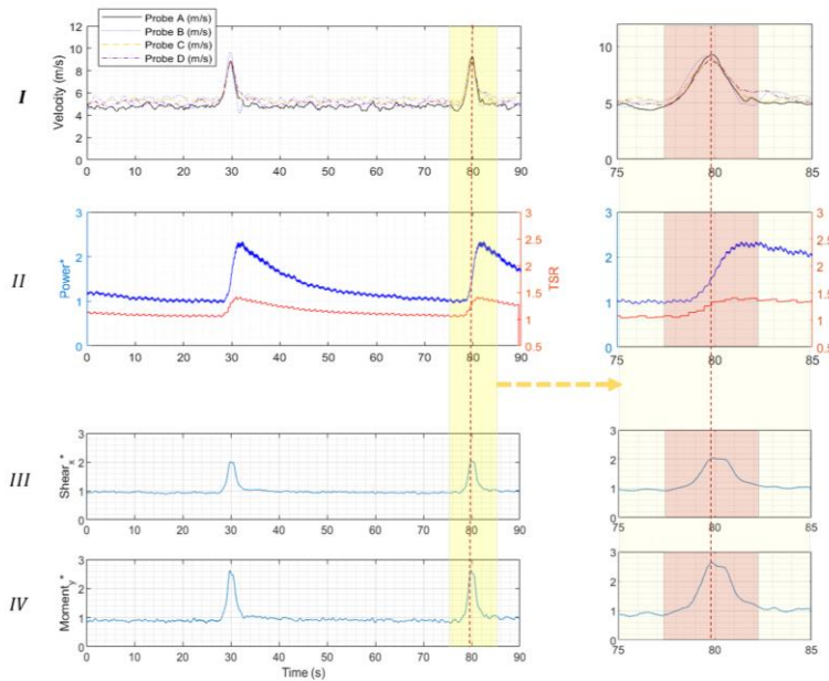
Figure 7.7: The time history of the results from all the probes in EOG using IGVs; Window I , the wind velocities from 4 cobra probes; Window II , power performance of the turbine; Windows III & IV , the forces X shear and moments Y moment at the tower base. The starred axis indexes are normalized by their corresponding value from uniform case B. 10 seconds window around the extreme events has been magnified and replotted at the right side with a red 5 seconds window highlighting the theoretical duration of the extreme event, and the red dashed line assumed as the center of the events which passes through the first velocity peak.
