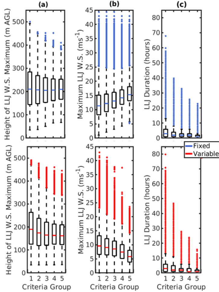
Fig 9. – Box-whisker plots for definition-wise distributions of spatiotemporal LLJ characteristics (a) jet core height; (b) jet core speed; and (c) jet duration over the entire domain. Note: the whiskers on the boxplots extend from the 75 th percentile to plus 1.5* times the inter-quartile range, and from the 25 th percentile to 1.5* times the inter-quartile range. Points beyond those values are defined as outliers and plotted as individual points.
