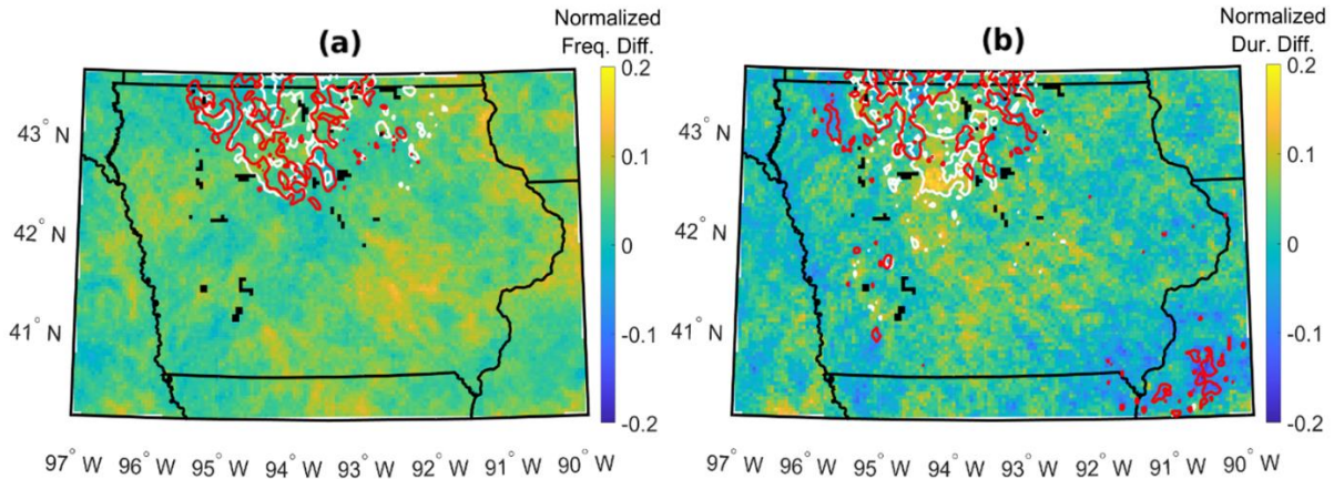
Fig 12. –Mean spatial results for Dec. 2007 – May 2008, inclusive. Maps colored by difference in (a) normalized LLJ frequency and (b) normalized LLJ duration for output at full resolution and down-sampled to 7 layers. Contours represent regions of highest 5% of (a) LLJ frequency and (b) LLJ duration for output at full resolution (white) and down-sampled to 7 layers (red).
