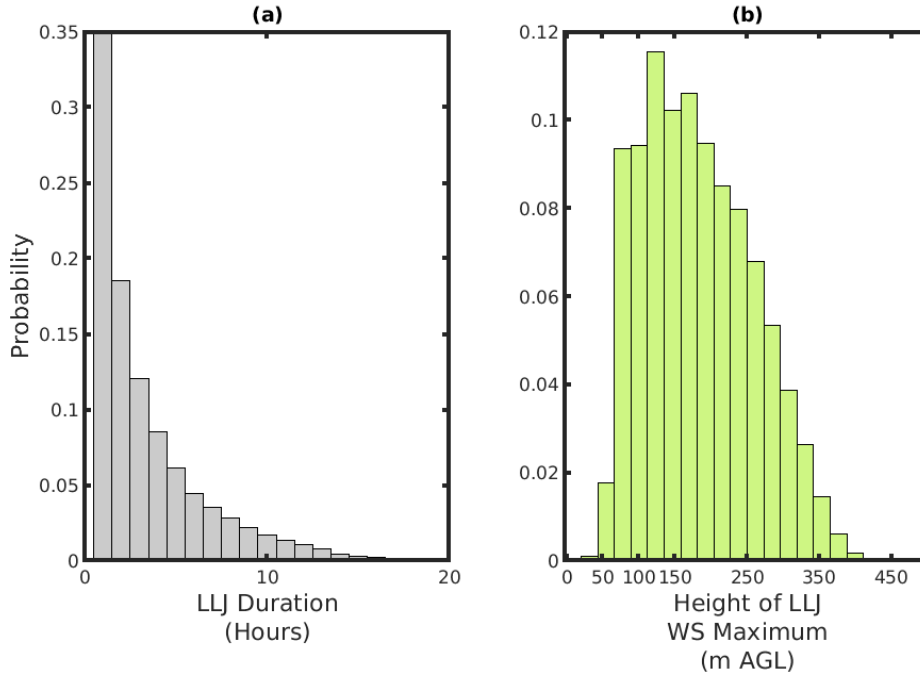
235 Fig 4. – Probability distributions from a domain-wide sample of all hourly realizations (n=4392) of vertical LLJ wind speed (WS) profiles for: (a) LLJ duration; (b) Height of the jet core. Note that LLJ with durations of over 20 hours were identified, but the distribution is truncated at 20 hours for legibility.
