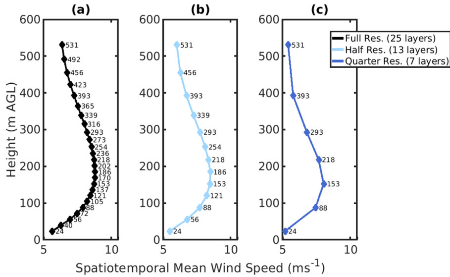
Fig 11. – Mean wind speed profiles for output at; (a) – full resolution (25 layers, no down-sampling); (b) – half resolution (13 layers, output down-sampled to every other layer); (c) – quarter resolution (7 layers, output down-sampled to every fourth layer). Note: layers are connected linearly for figure visibility, but the LLJ wind speed maxima can only occur at the heights defined at the vertical layers (25, 13, and 7 heights respectively for each resolution).
