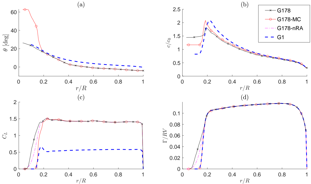
Figure 3. Twist Distributions of twist \theta (a), non-dimensional chord c/c_0 (b), lift coefficient C_L (c), and non-dimensional circulation \Gamma/RV distributions (d), for the G1 and for the G178, G178-MC, and G178-nRA full-scale turbines.
