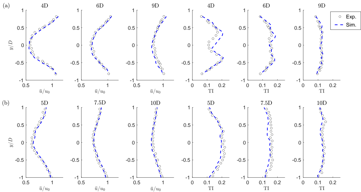
Figure 8. Horizontal hub-height profiles of normalized time-average streamwise velocity and turbulence intensity, for the medium (a) and high (b) inflow TI cases. Black o symbols: experimental results; blue dashed line: G1 simulations.
