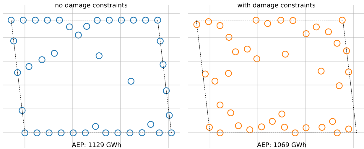
Figure 15. The optimal layout results from our optimization. On the left are the optimal turbine locations when the turbine layout is optimized without damage constraints. On the right are the turbine locations when damage from partial waking is constrained to be less than 0.04. The dotted black lines represent the wind farm boundary and the circles represent the wind turbines, with the circle diameter accurately scaled to represent the turbine rotor diameter.
