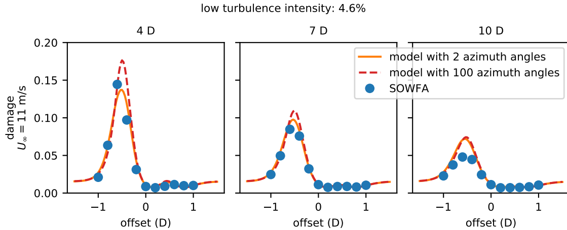
Figure 9. Final damage plots calculated with different numbers of azimuth angle evaluations. The orange line represents damage calculated with 2 azimuth angle evaluations at 90 and 270 degrees, the dashed red line represents the damage calculated with 100 azimuth angle evaluations, and the blue points show the damage calculated with the high-fidelity SOWFA data.
