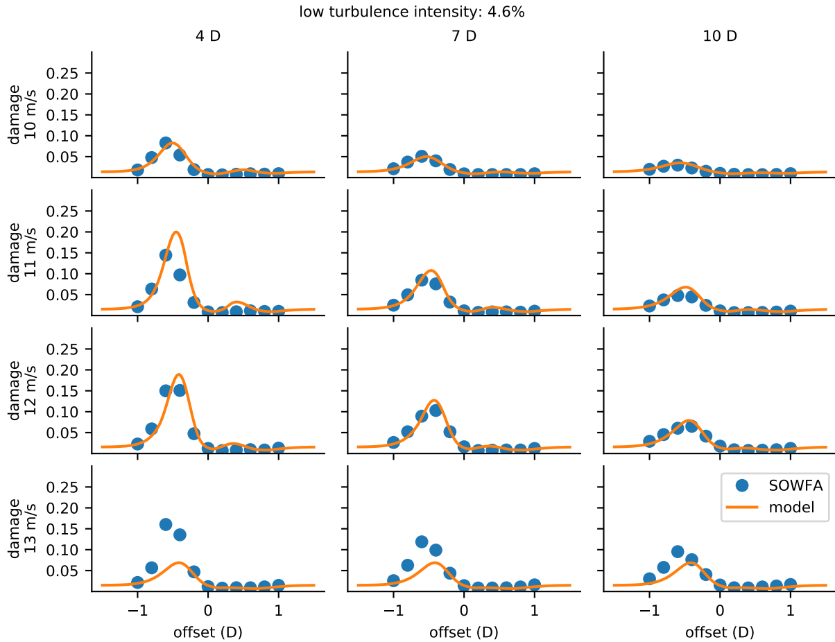
Figure 10. Comparison of our presented damage model to the lifetime damage predicted by the loads from the SOWFA and OpenFAST data. This figure is for a low freestream turbulence intensity of 4.6%. From top to bottom, each row represents different freestream wind speeds of 10, 11, 12, and 13 meters per second. From left to right, each column represents different distances from the upstream turbine of 4 D, 7 D, and 10 D.
