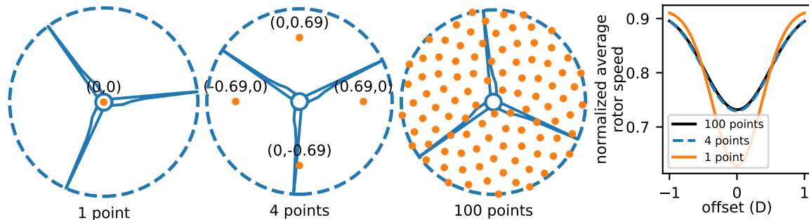
Figure 6. The sample points used to calculate the average wind speed into a turbine. From left to right, the location of the 1, 4, and 100 sample points are shown on the swept area of the rotor. On the far right: the average rotor speed of a turbine moving across the wake of an upstream turbine. The downstream turbine moves from one side of the wake (-1 D offset) to the other side of the wake (1 D offset). Each of the 3 lines shows the average rotor wind speed calculated with 1, 4, and 100 sample points.
