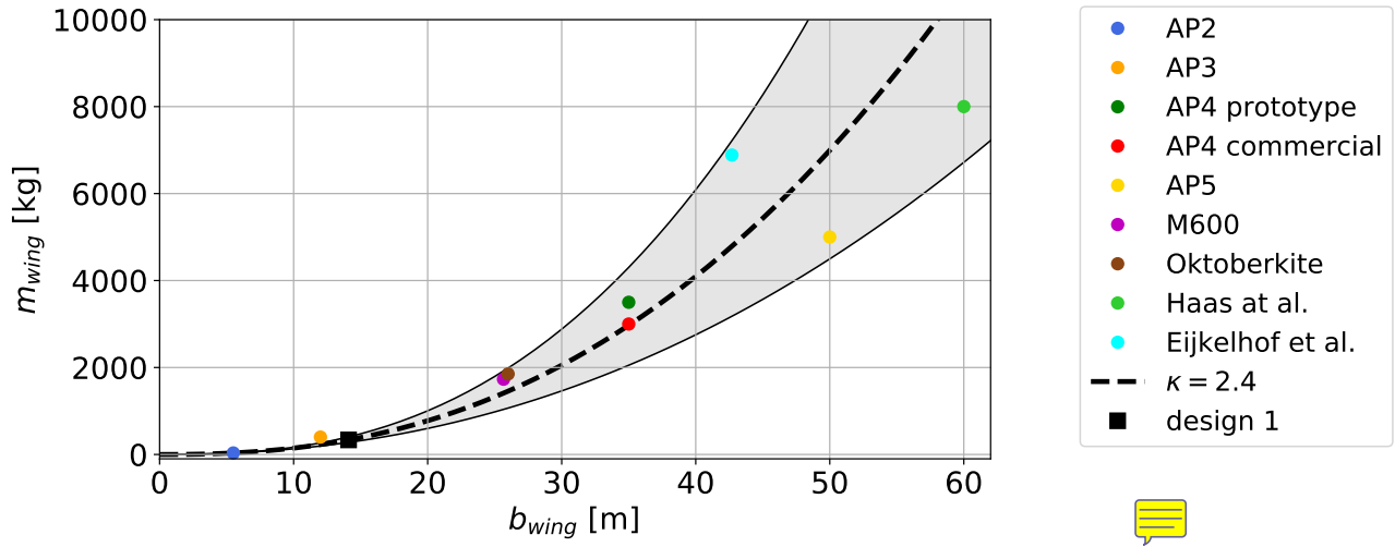
Figure 10. Curve fit of published sizing study ies AWES aircraft mass (Haas et al., 2019; Kruijff and Ruiterkamp, 2018; Eijkelhof et al., 2020; Ampyx, 2020; Echeverri et al., 2020). For these data mass scales within a scaling exponent range of \kappa = 2.2 - 2.6 (grey area). The chosen mass scaling exponent of \kappa = 2.4 is represented by a dashed line and the modeled design 1 is highlighted by a black square.
