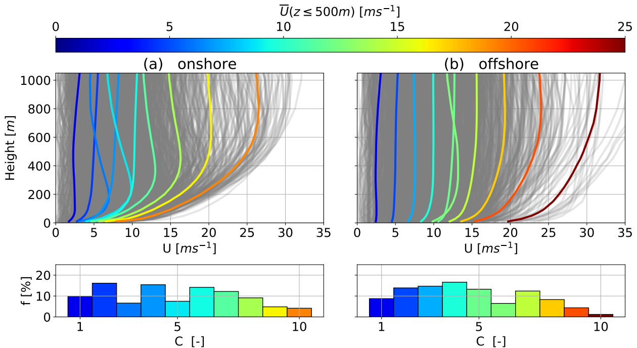
Figure 5. Onshore (left) and offshore (right) average annual wind speed profiles (or centroids) resulting from the k -means clustering process for k = 10 over height (top). Comprising WRF simulated wind velocity profiles depicted in grey. Centroids are sorted, labeled and colored in ascending order of average wind speed up to 500 m. The corresponding cluster frequency f for each cluster C is shown below.
