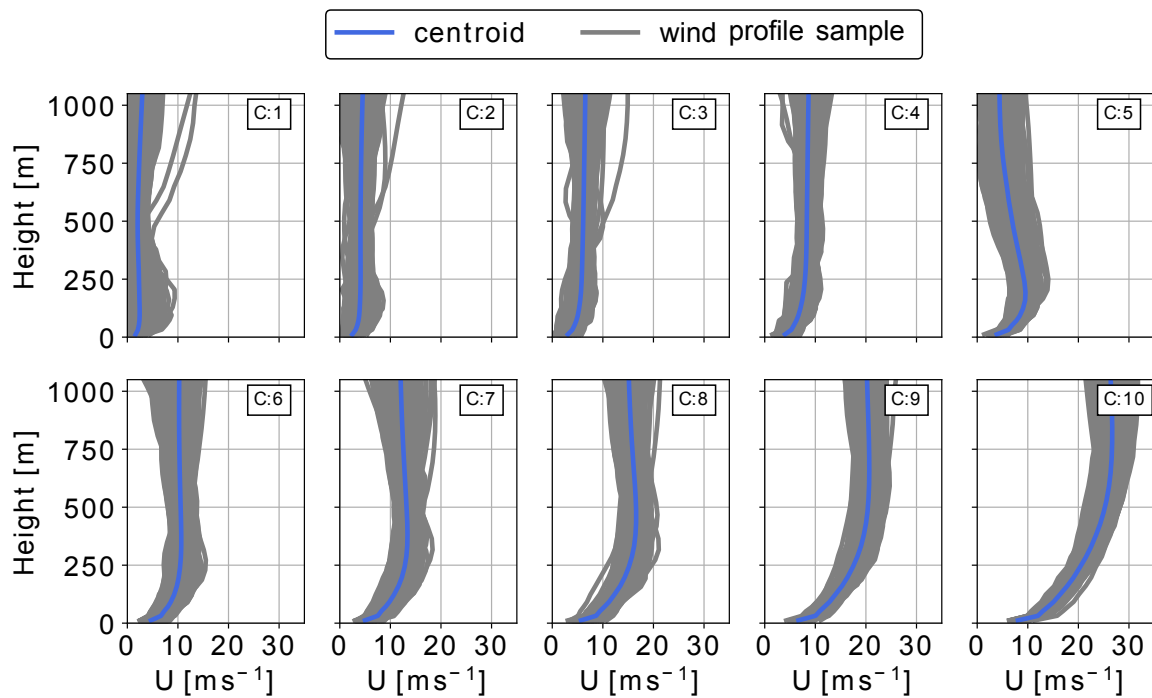
Figure A2. Clustered onshore wind velocity profiles (here shown as projected wind speed profiles). The average profile or centroid is shown in blue while all the assigned profiles are shown in grey.
