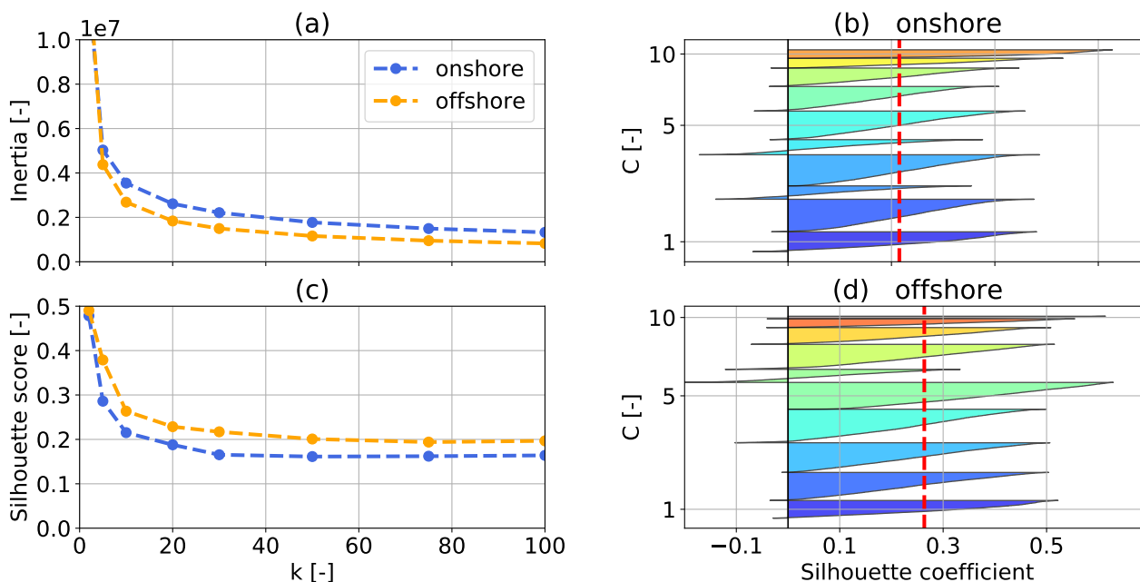
Figure 4. k -means clustering inertia over number of cluster k (a) for one year of onshore (blue) and offshore (orange) wind velocity profiles up to 1000 m. Silhouette score (c), average silhouette coefficients, over number number of cluster k for both locations. Onshore (b) and offshore (d) silhouette coefficients ( k=10 ) express the distance to neighbouring clusters. The red dashed line represents the silhouette score.
