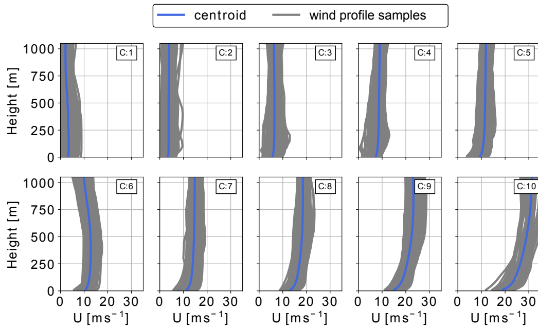
Figure A1. Clustered offshore wind velocity profiles (here shown as C 2D vertical projected wind speed profiles). The average profile or centroid is shown in blue while all the assigned profiles are shown in grey.
