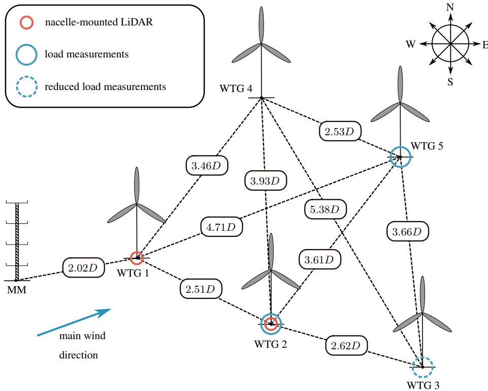
Figure 1. Wind farm layout with measurement equipment (Reinhardt et al., 2020).
