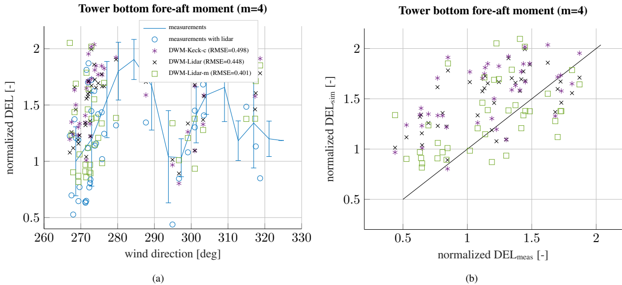
Figure 17. Measured and simulated tower bottom fore-aft bending moment over the wind direction (a) and simulated loads over measured loads (b) at an ambient wind speed of 8 m/s and an ambient turbulence intensity of 10 %, when WTG 2 is exposed to the wake of WTG 1.
