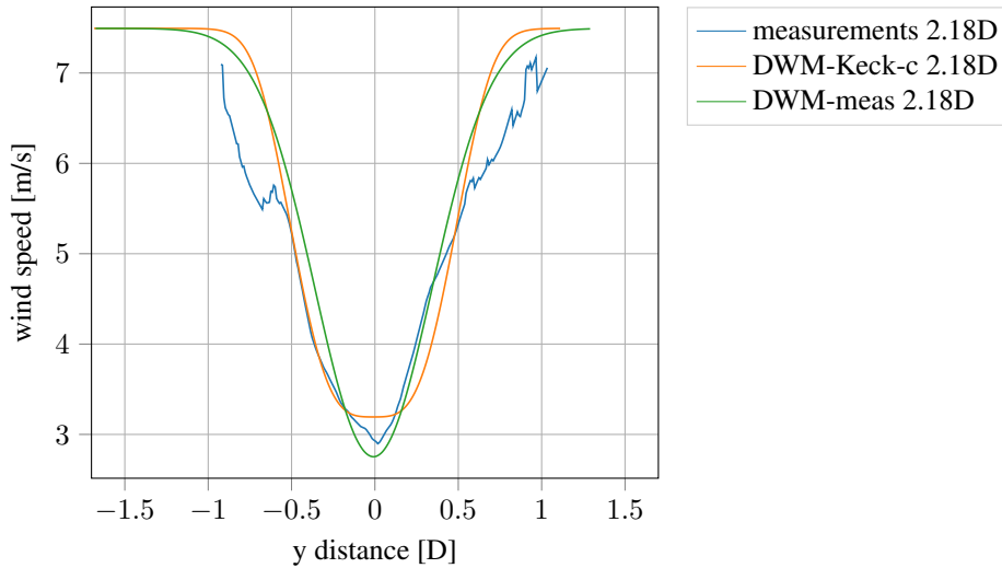
Figure 6. Wind speed deficit in the HMFR; measured and simulated with the calibrated DWM-Keck-c model as well as fitted to a Gaussian shaped wake model (DWM-meas).
