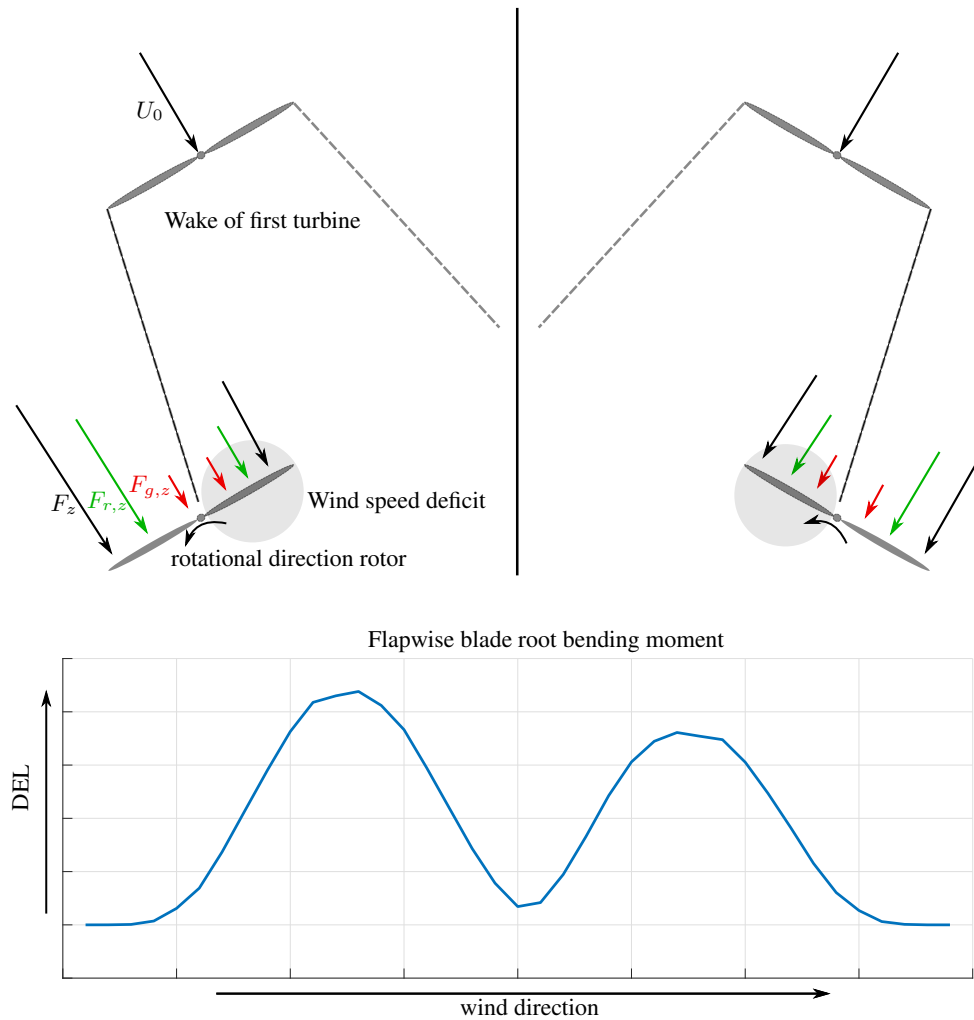
Figure A1. Schematic illustration of the flapwise blade root bending moment according to Reinhardt (2017). The aerodynamic force F_{r,z} , the gravitational force F_{g,z} , as well as the total force F_z perpendicular to the rotor plane at different wake situations are marked.
