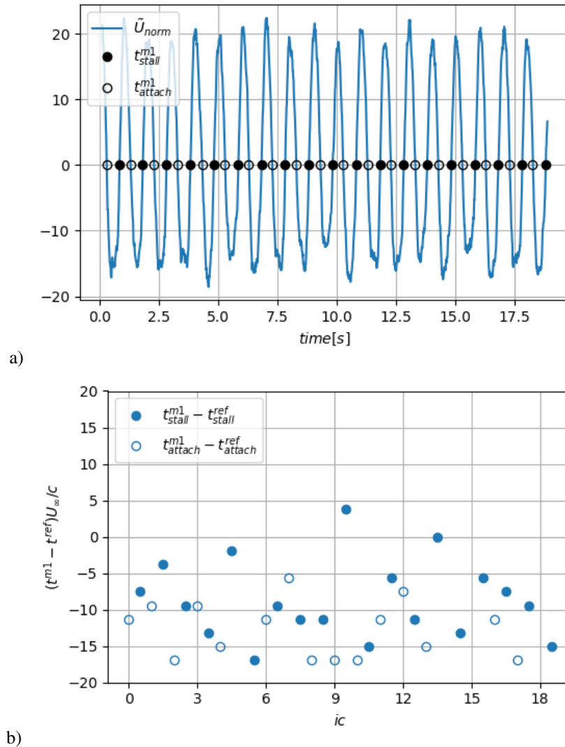
Figure 16. Results from the zero-crossing method applied on the U_{norm}(t) signal: a) instantaneous signals with detected instants, b) Normalized delay of the stall and reattachment detected instants
